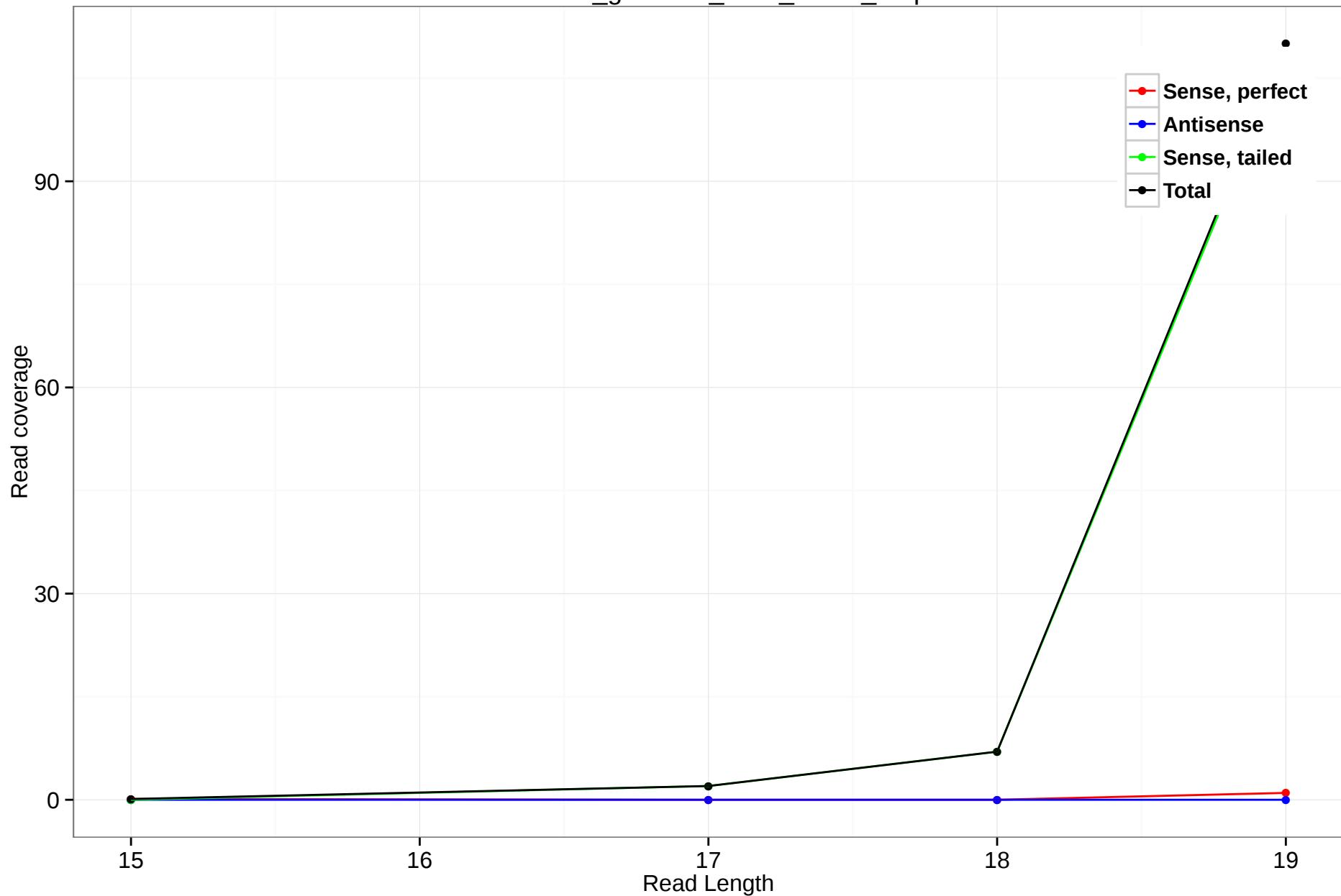
rheMac3_genscan_chrX_294.5_5.5p
