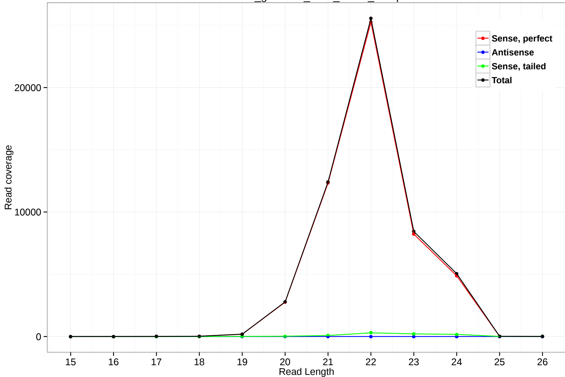
rheMac3_genscan_chrX_271.6_10.5p
