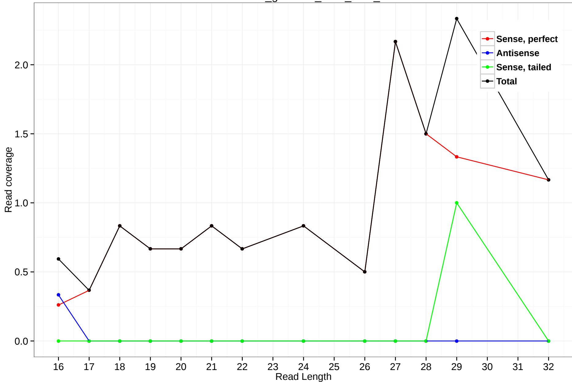
rheMac3_genscan_chrX_24.9_1
