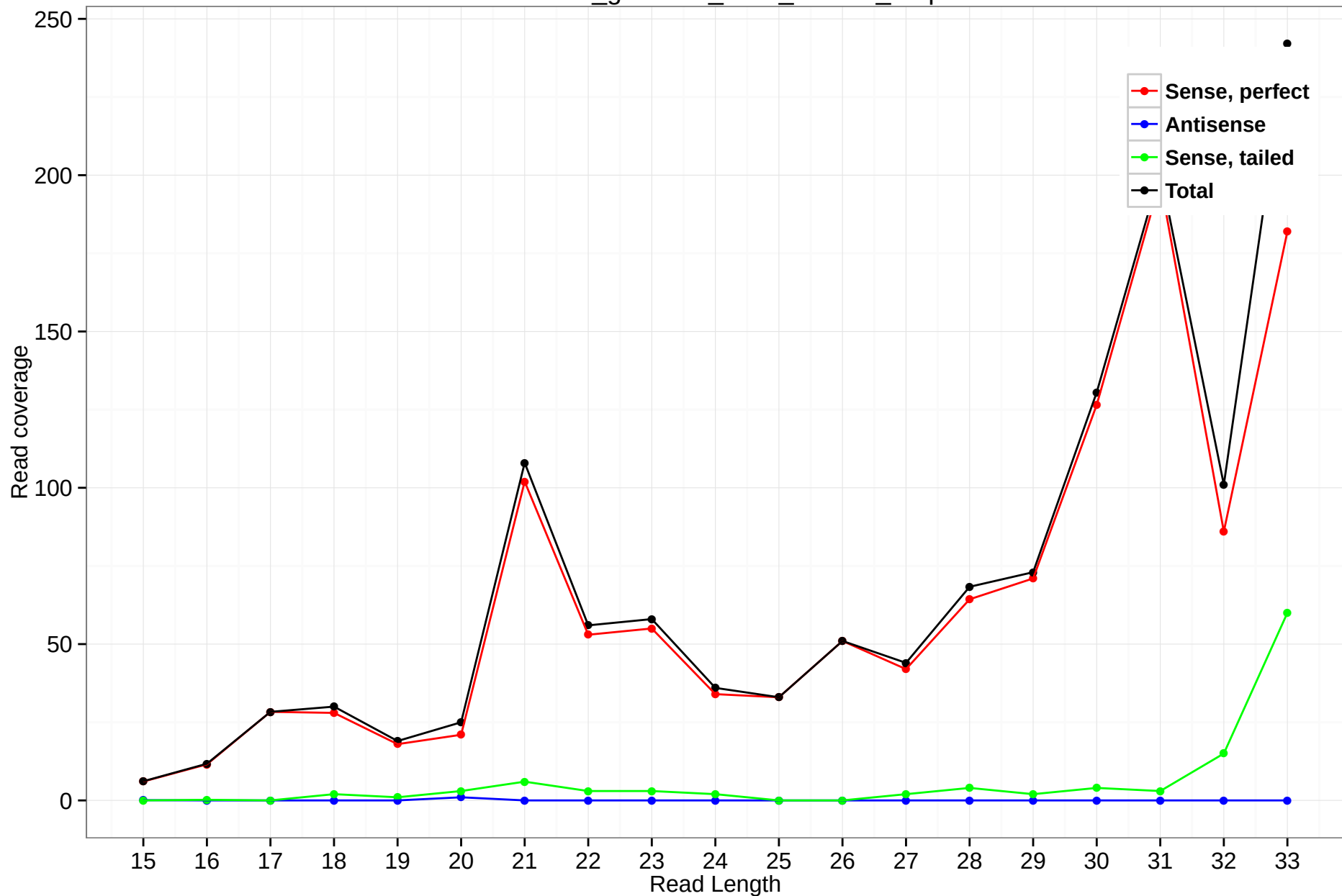
rheMac3_genscan_chrX_237.19_1.3p
