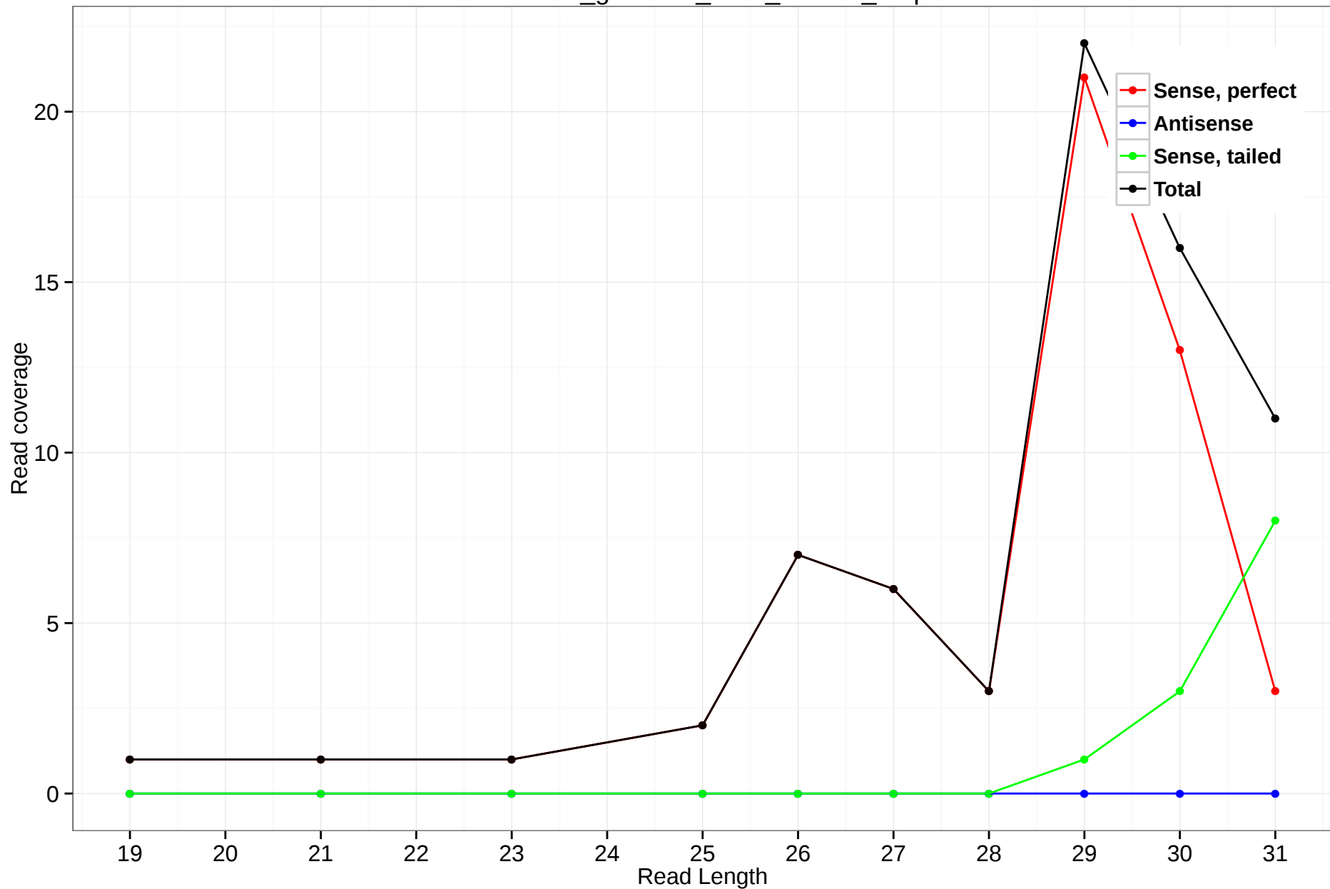
rheMac3_genscan_chrX_235.12_4.5p
