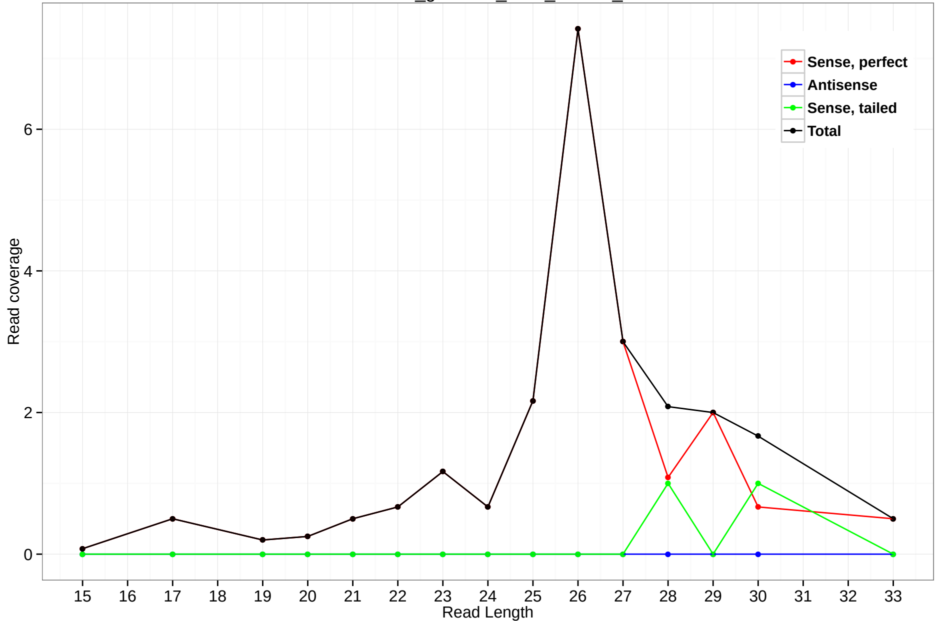
rheMac3_genscan_chrX_226.18_0
