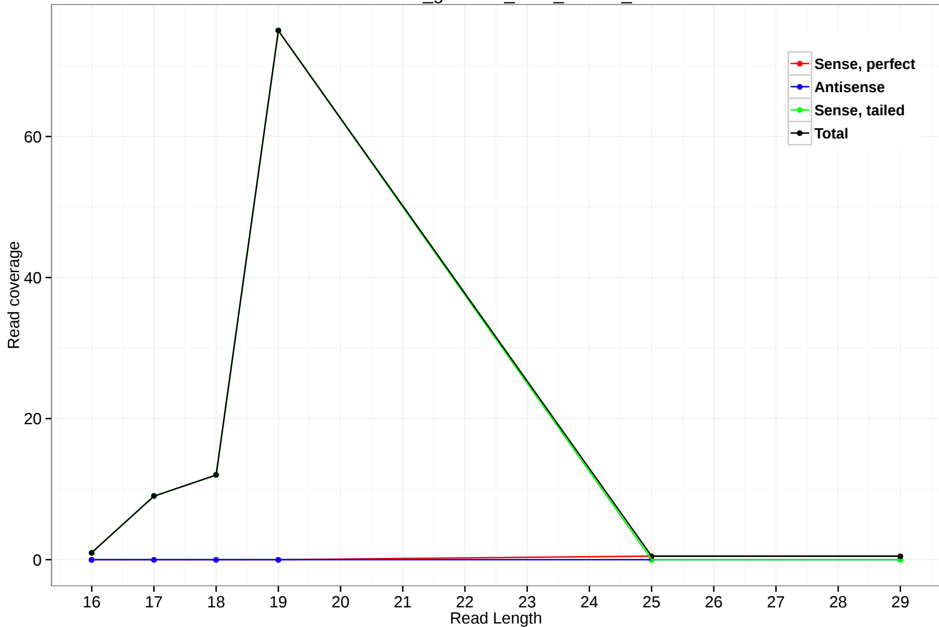
rheMac3_genscan_chrX_218.13_0
