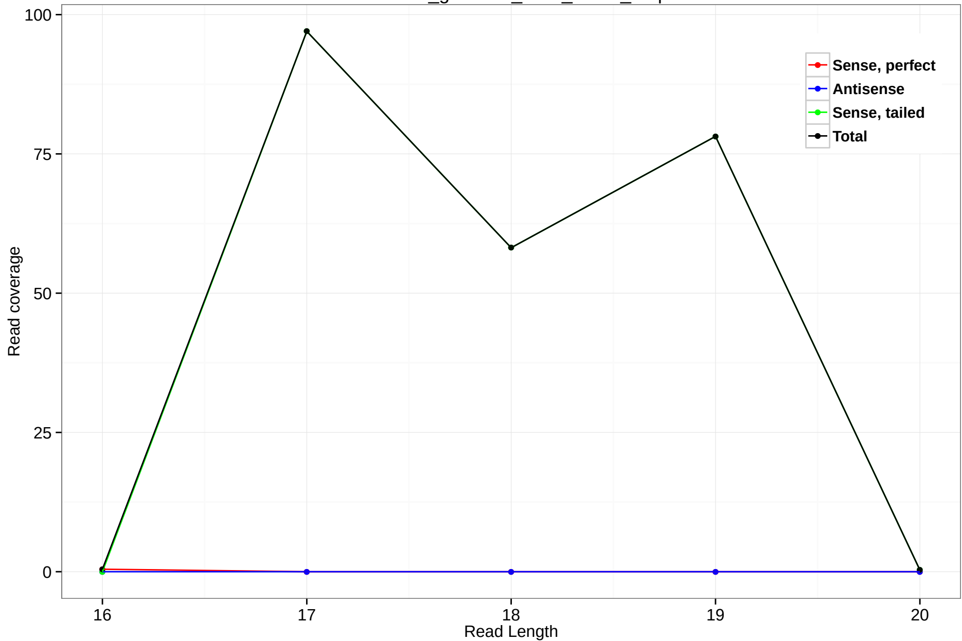
rheMac3_genscan_chrX_203.1_1.5p
