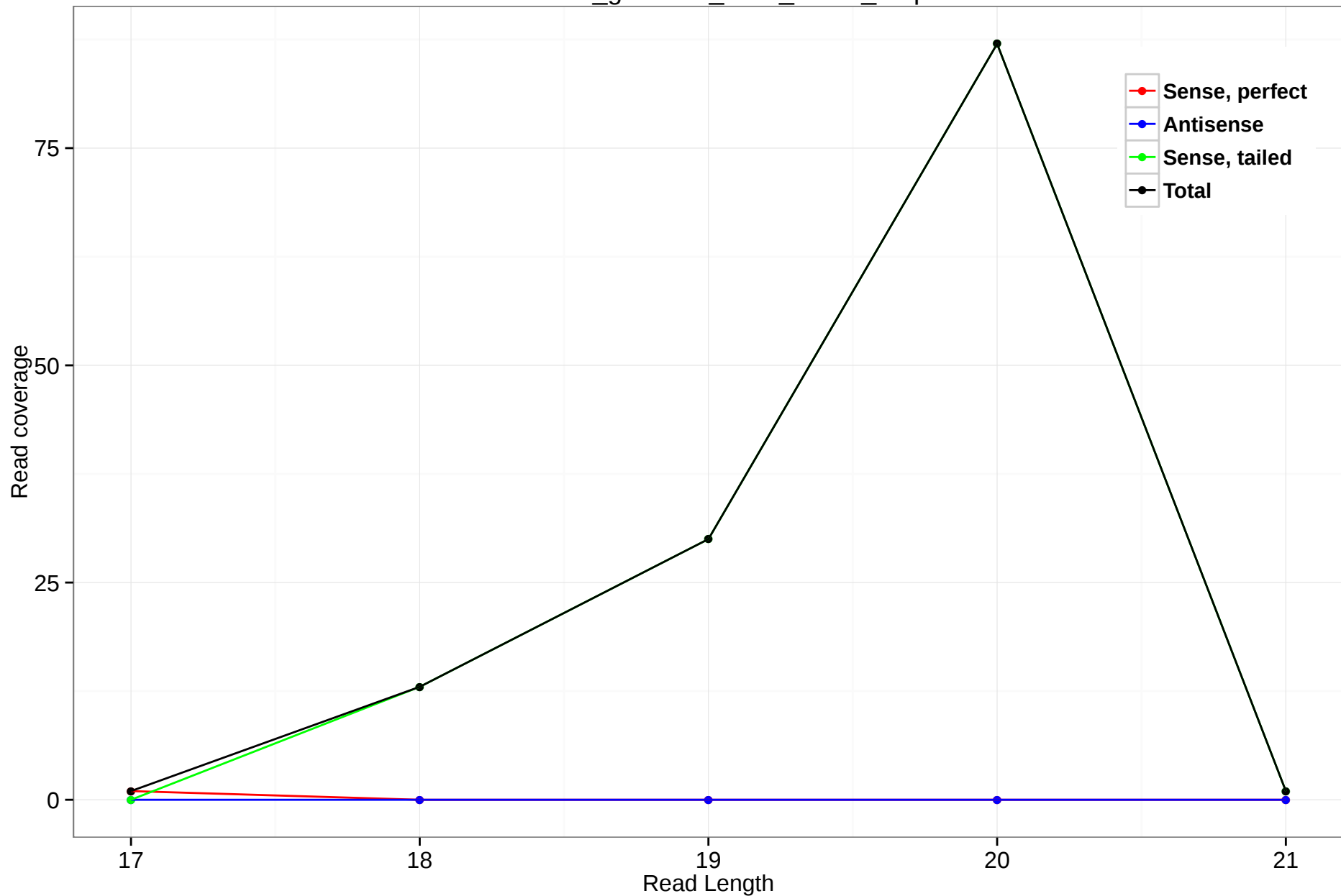
rheMac3_genscan_chrX_160.5_0.3p
