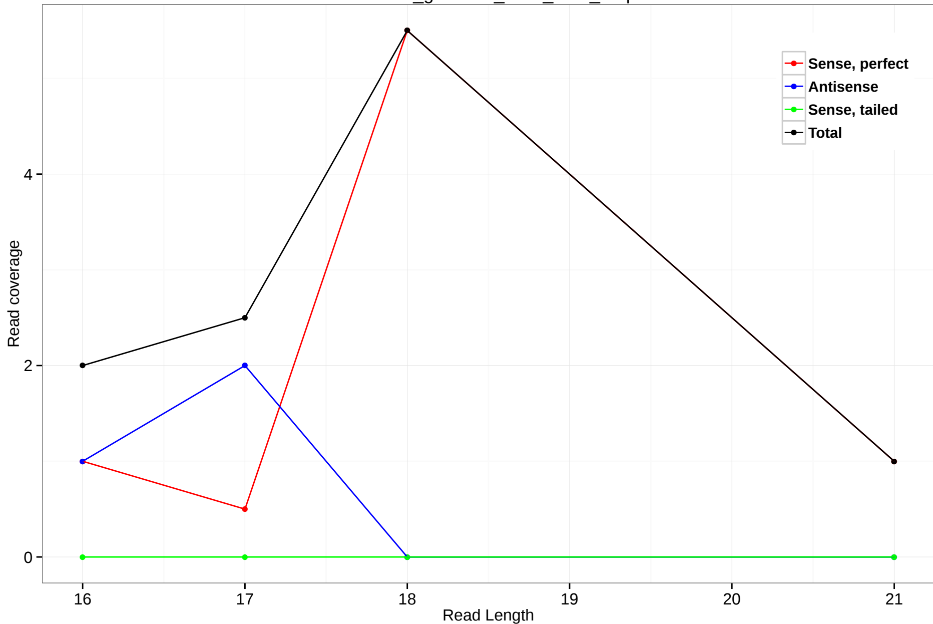
rheMac3_genscan_chrX_16.9_2.5p
