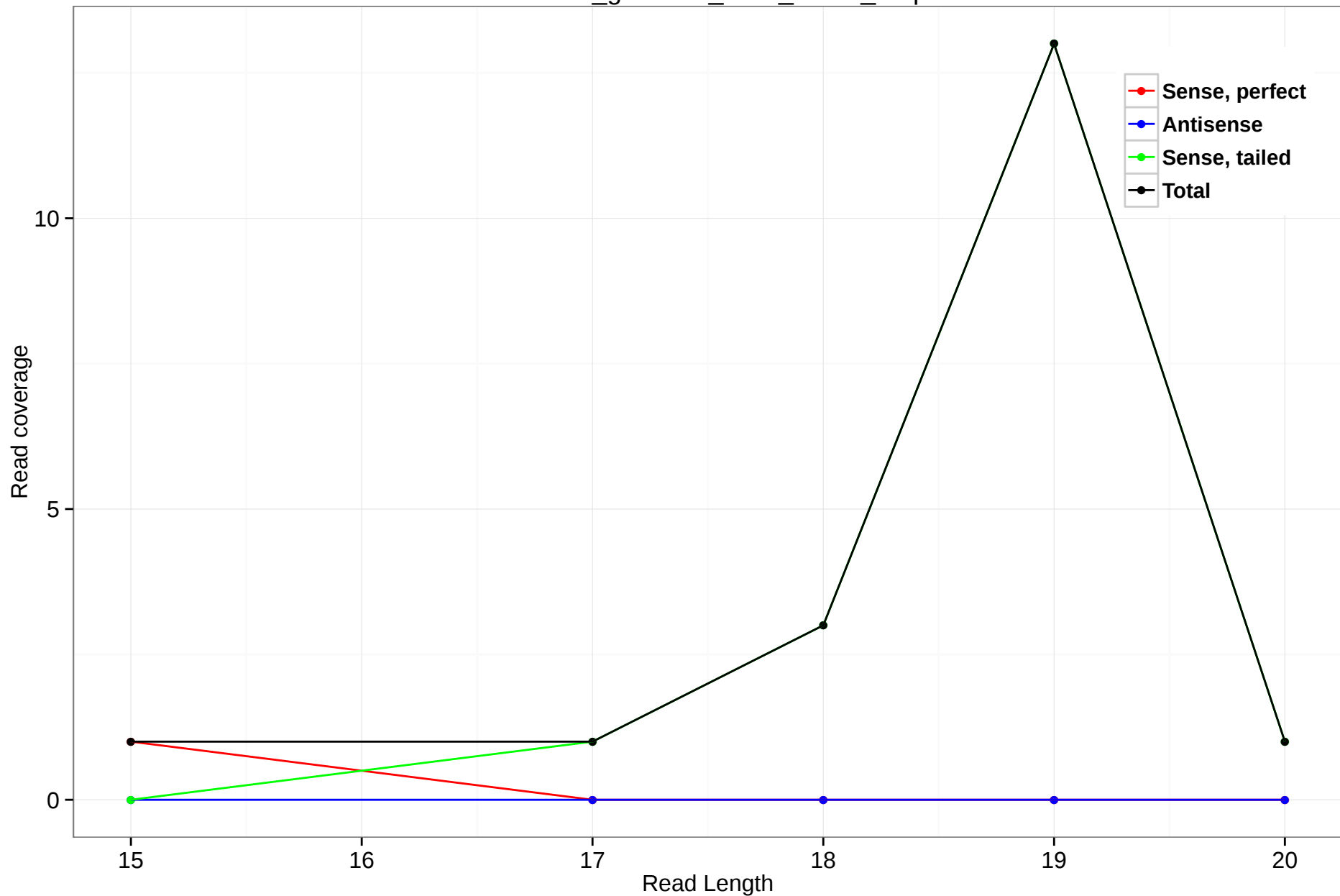
rheMac3_genscan_chrX_16.28_9.5p
