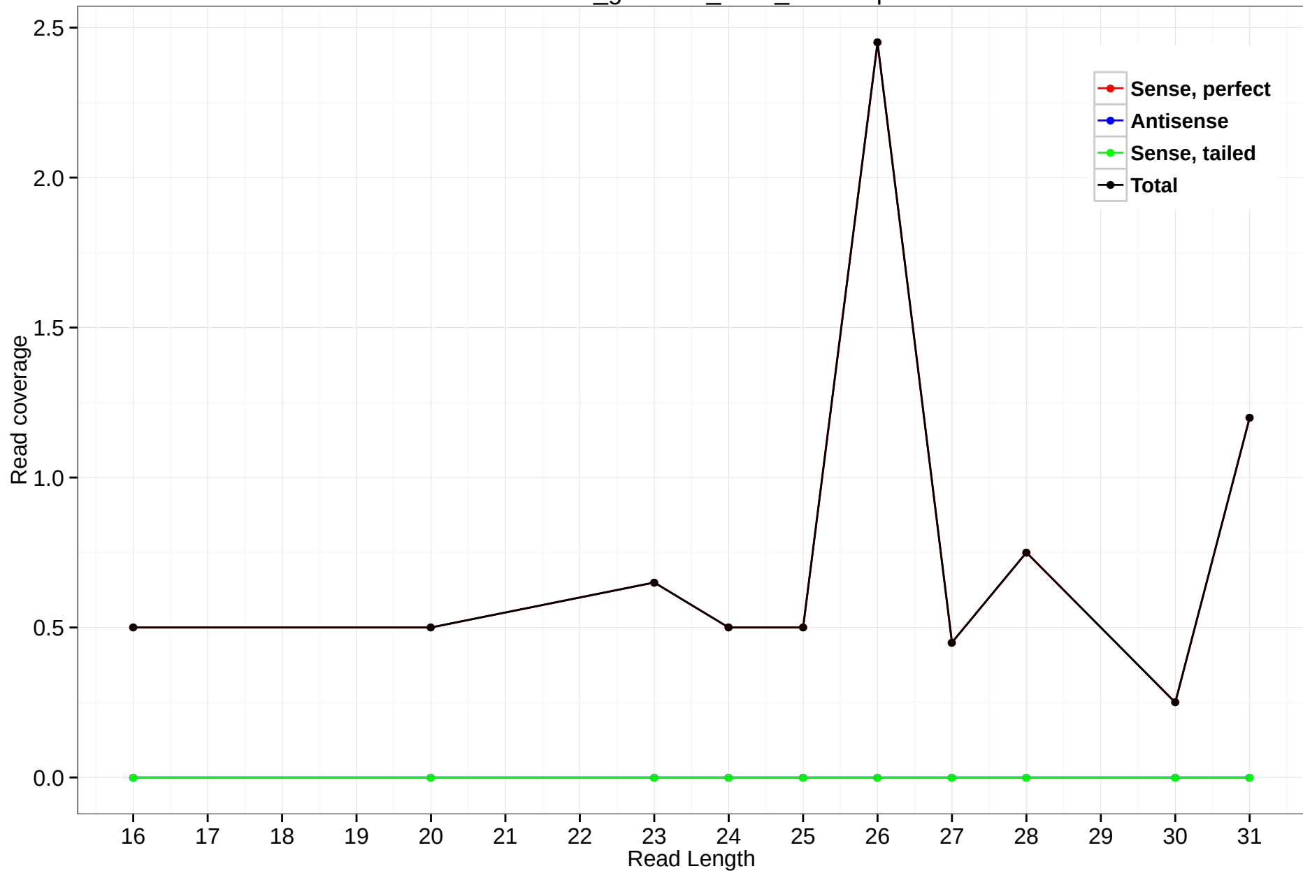
rheMac3_genscan_chrX_129.7.5p
