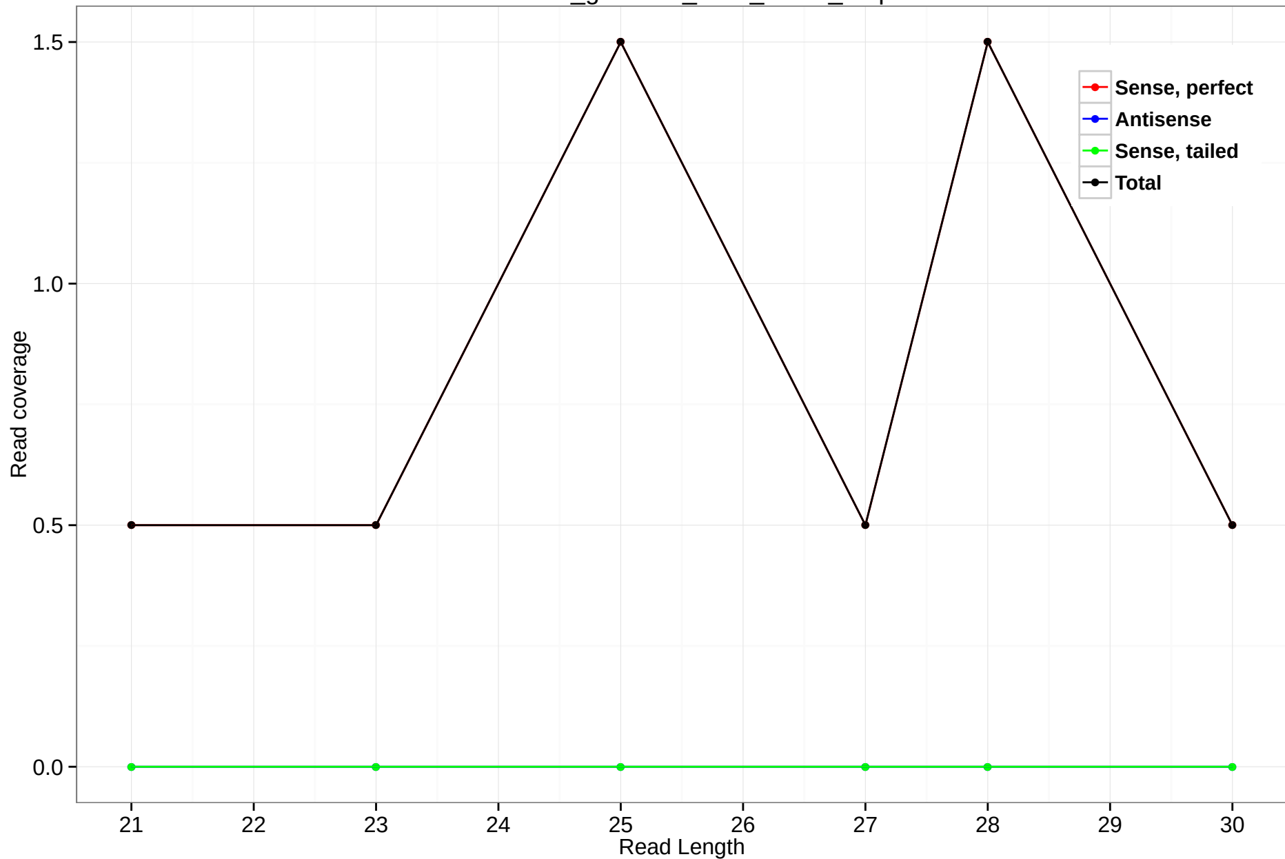
rheMac3_genscan_chrX_127.2_1.3p
