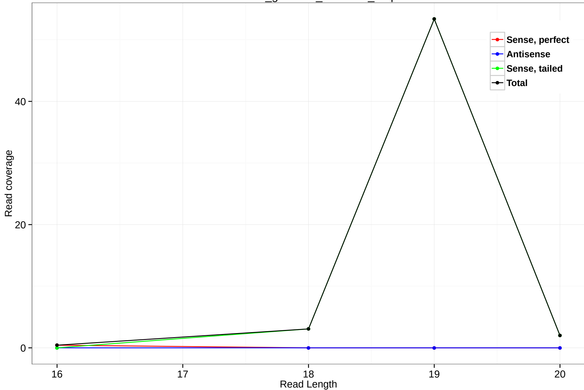
rheMac3_genscan_chr9.980_4.5p
