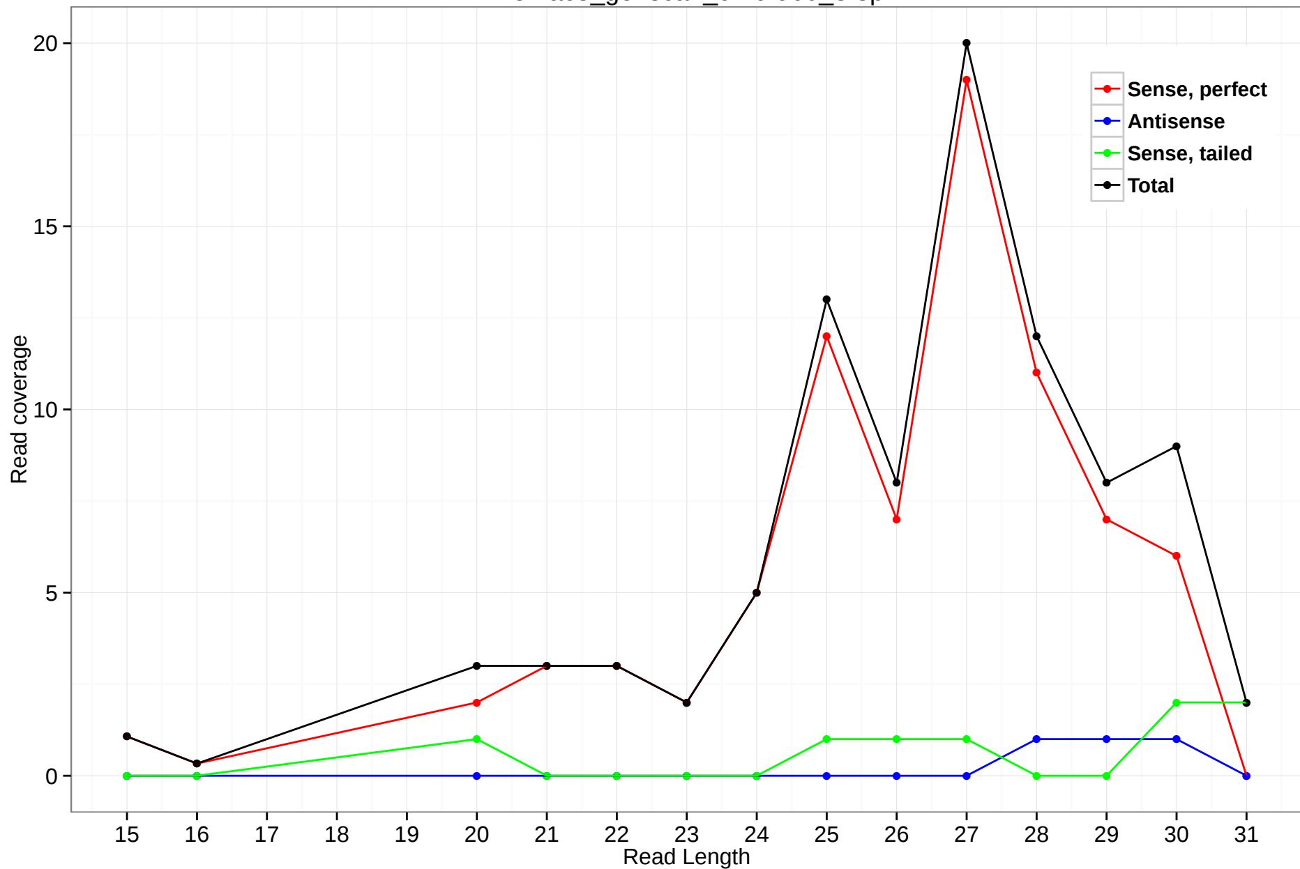
rheMac3_genscan_chr9.960_8.3p
