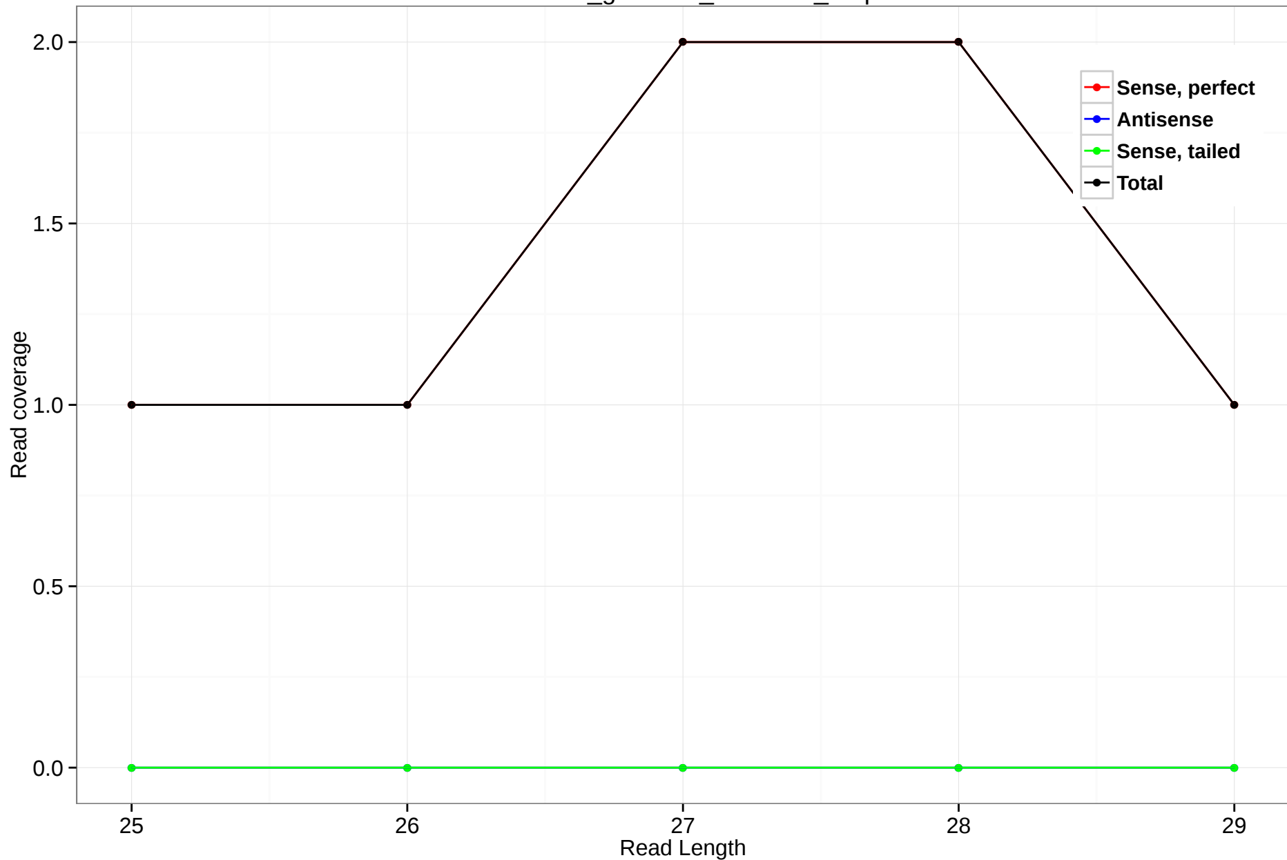
rheMac3_genscan_chr9.960_6.3p
