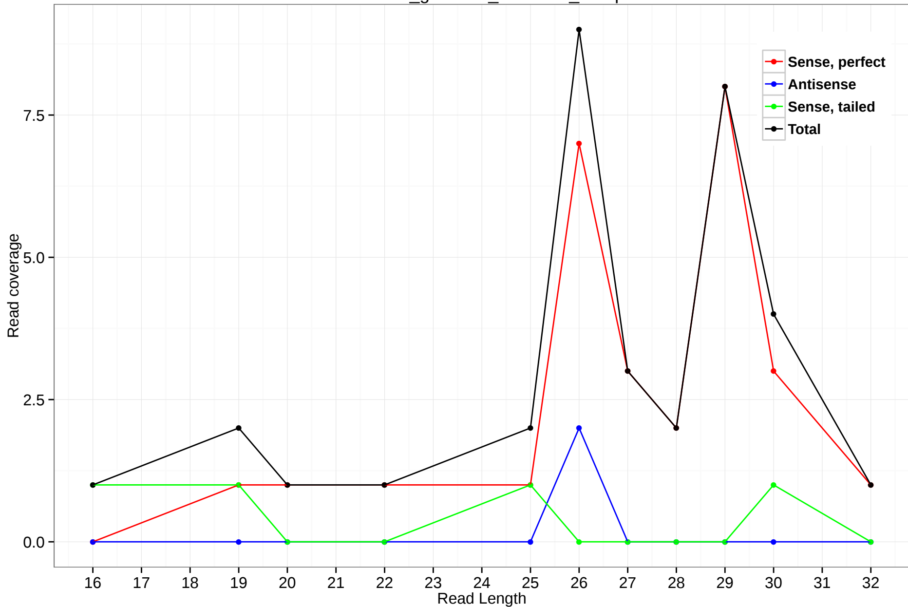
rheMac3_genscan_chr9.960_10.5p
