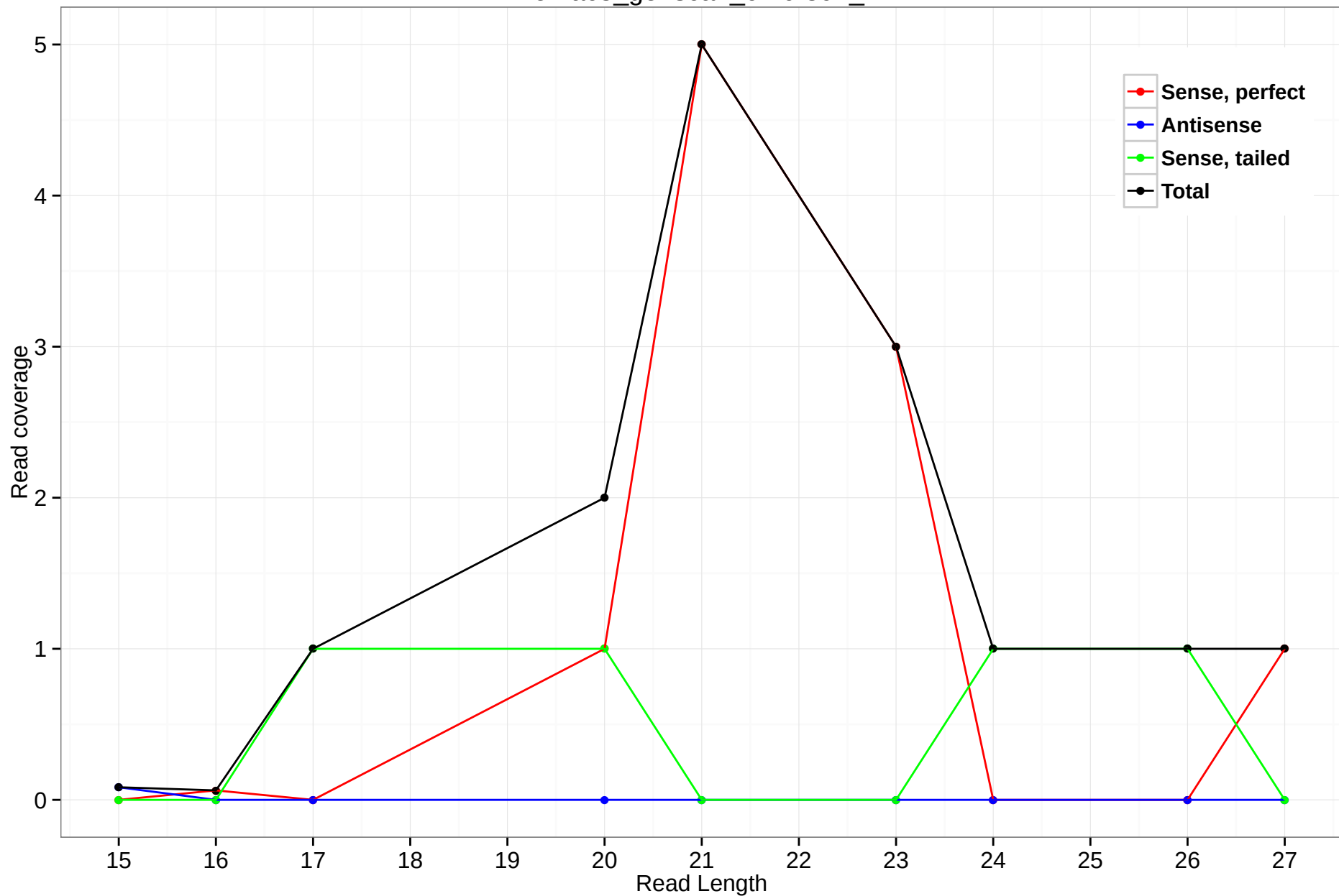
rheMac3_genscan_chr9.891_11
