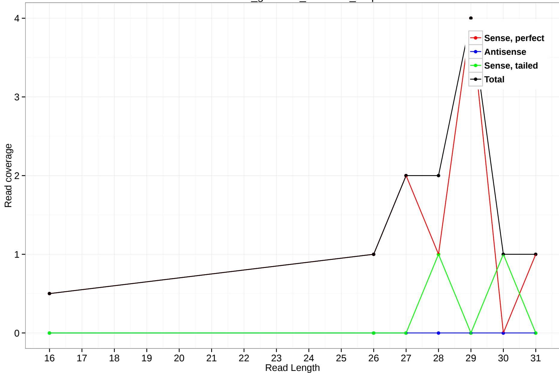
rheMac3_genscan_chr9.883_6.5p
