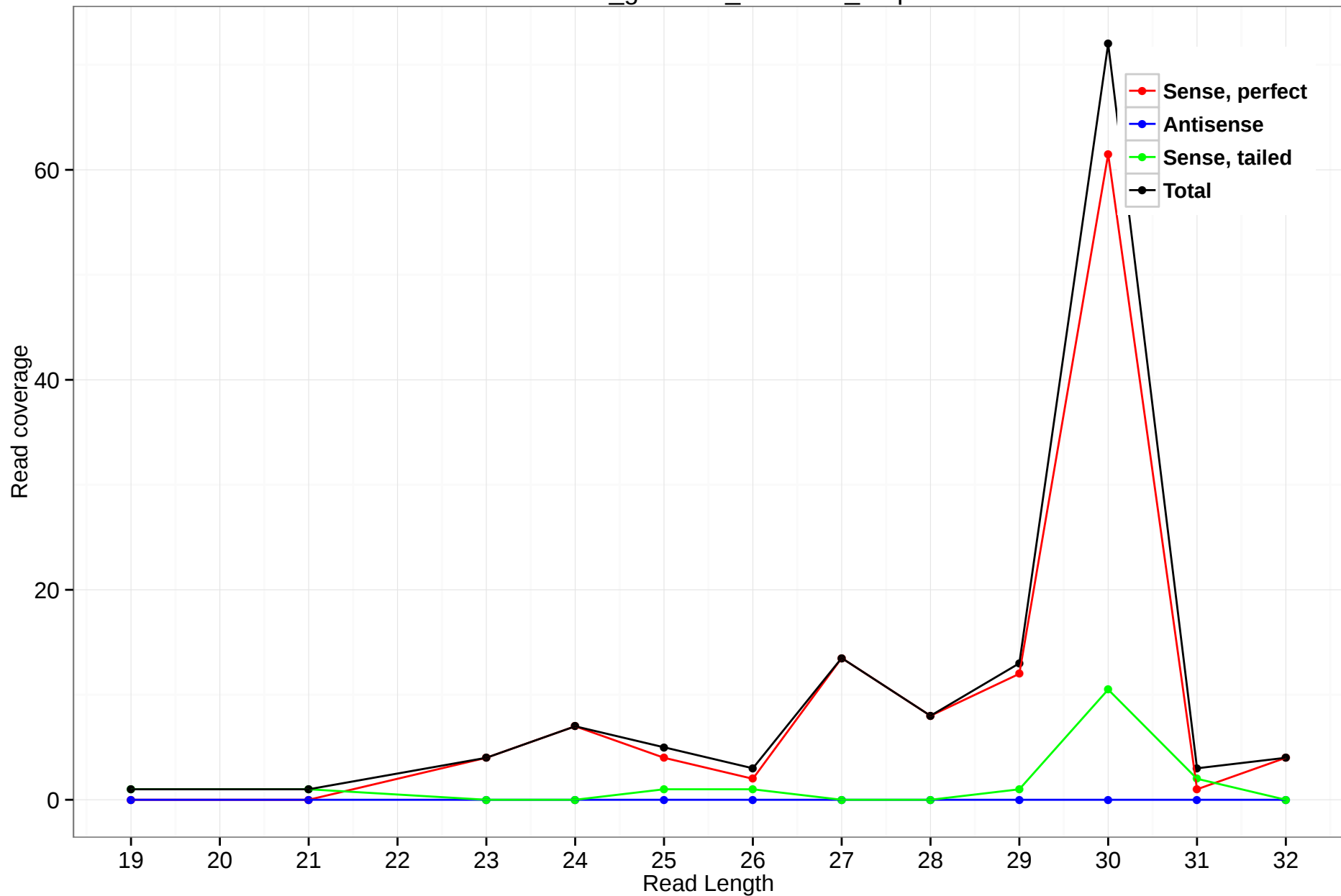
rheMac3_genscan_chr9.883_4.5p
