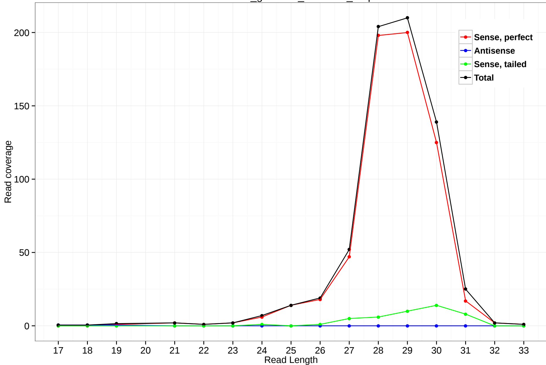
rheMac3_genscan_chr9.883_3.5p
