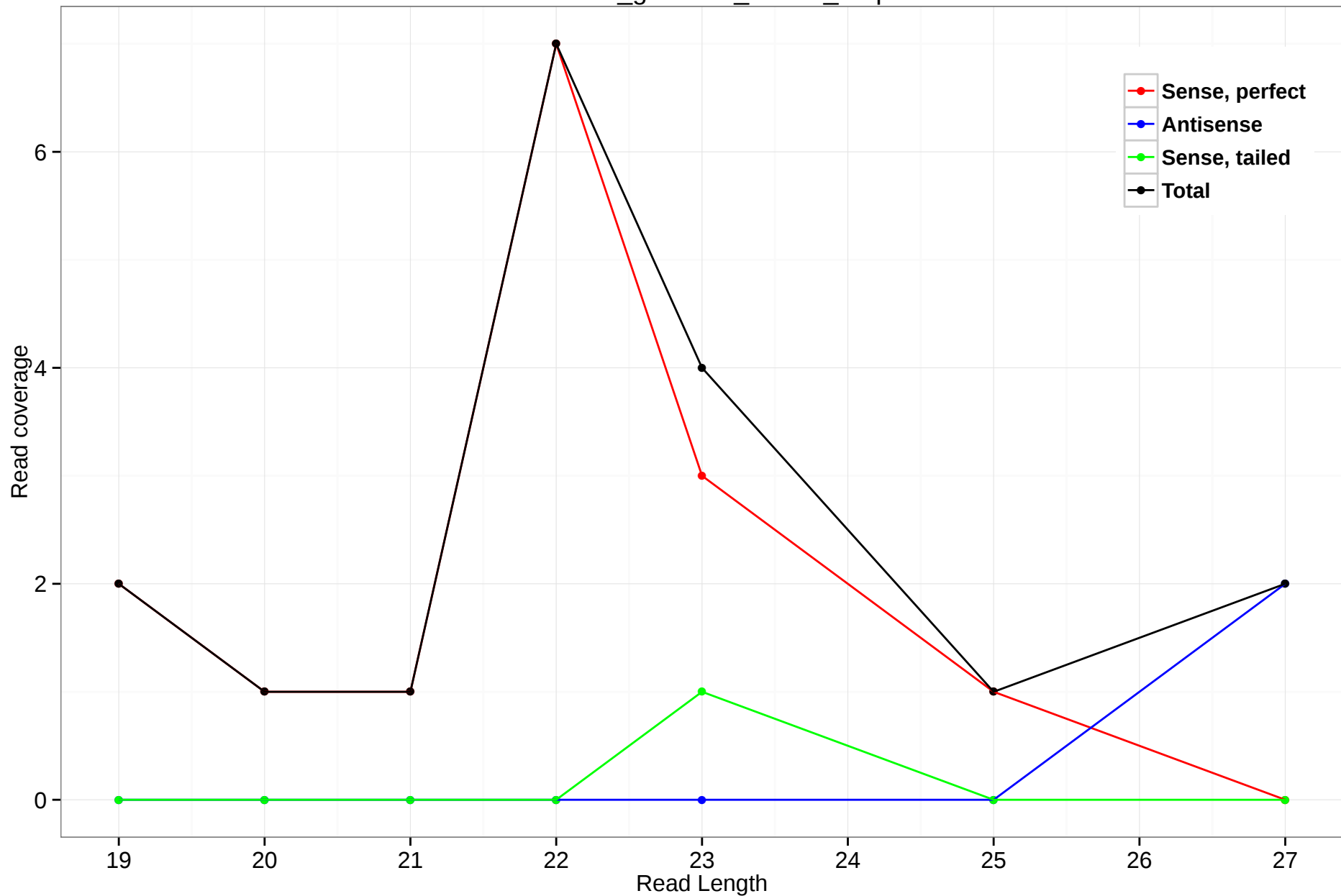
rheMac3_genscan_chr9.7_1.3p
