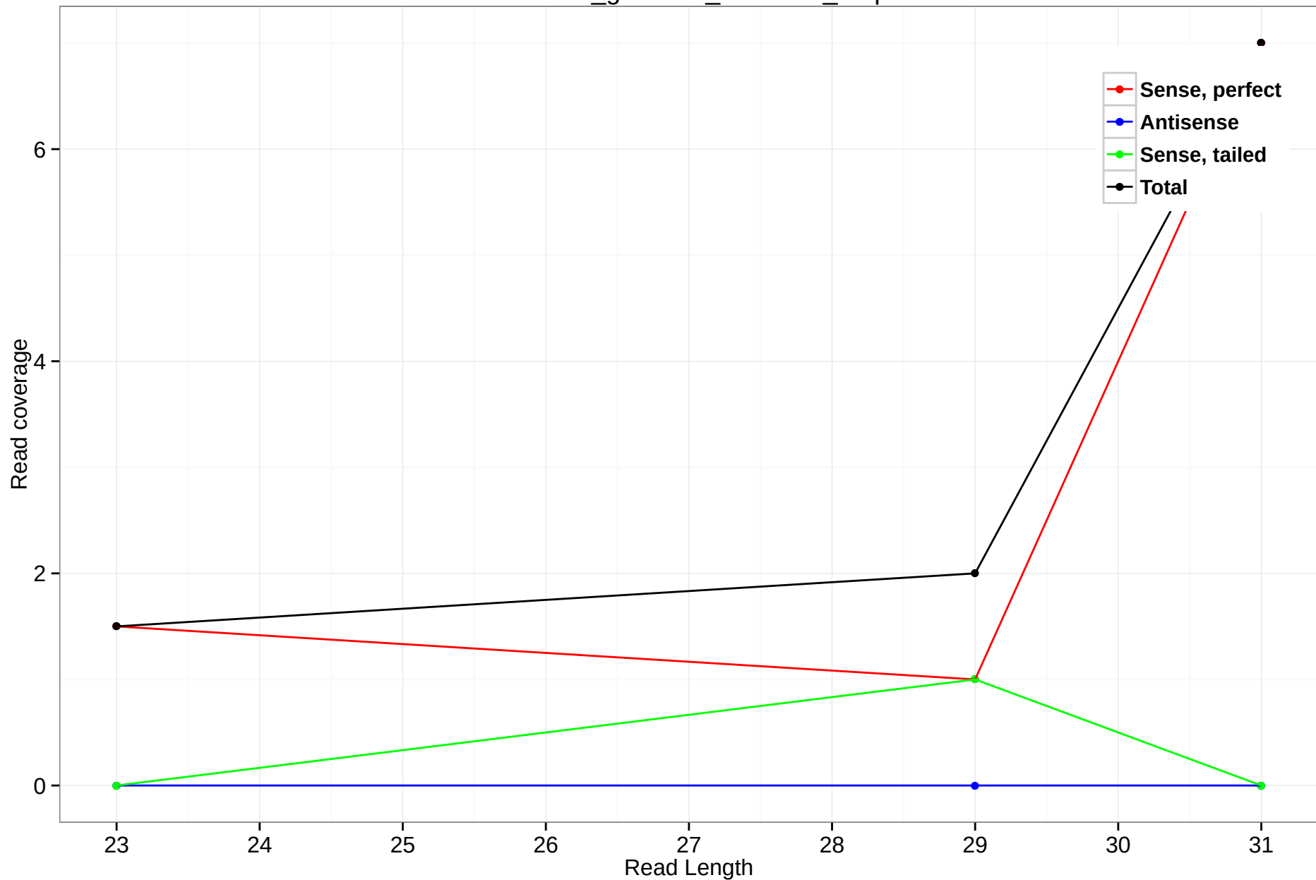
rheMac3_genscan_chr9.760_2.5p
