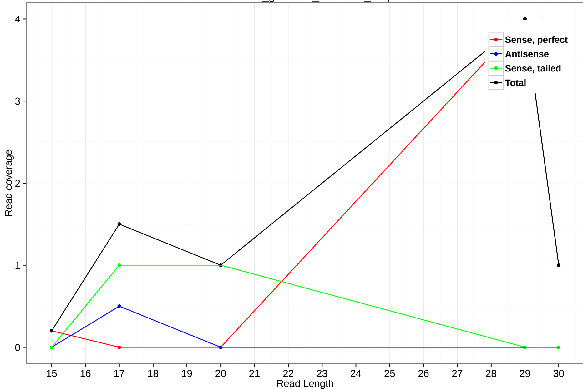
rheMac3_genscan_chr9.749_0.3p
