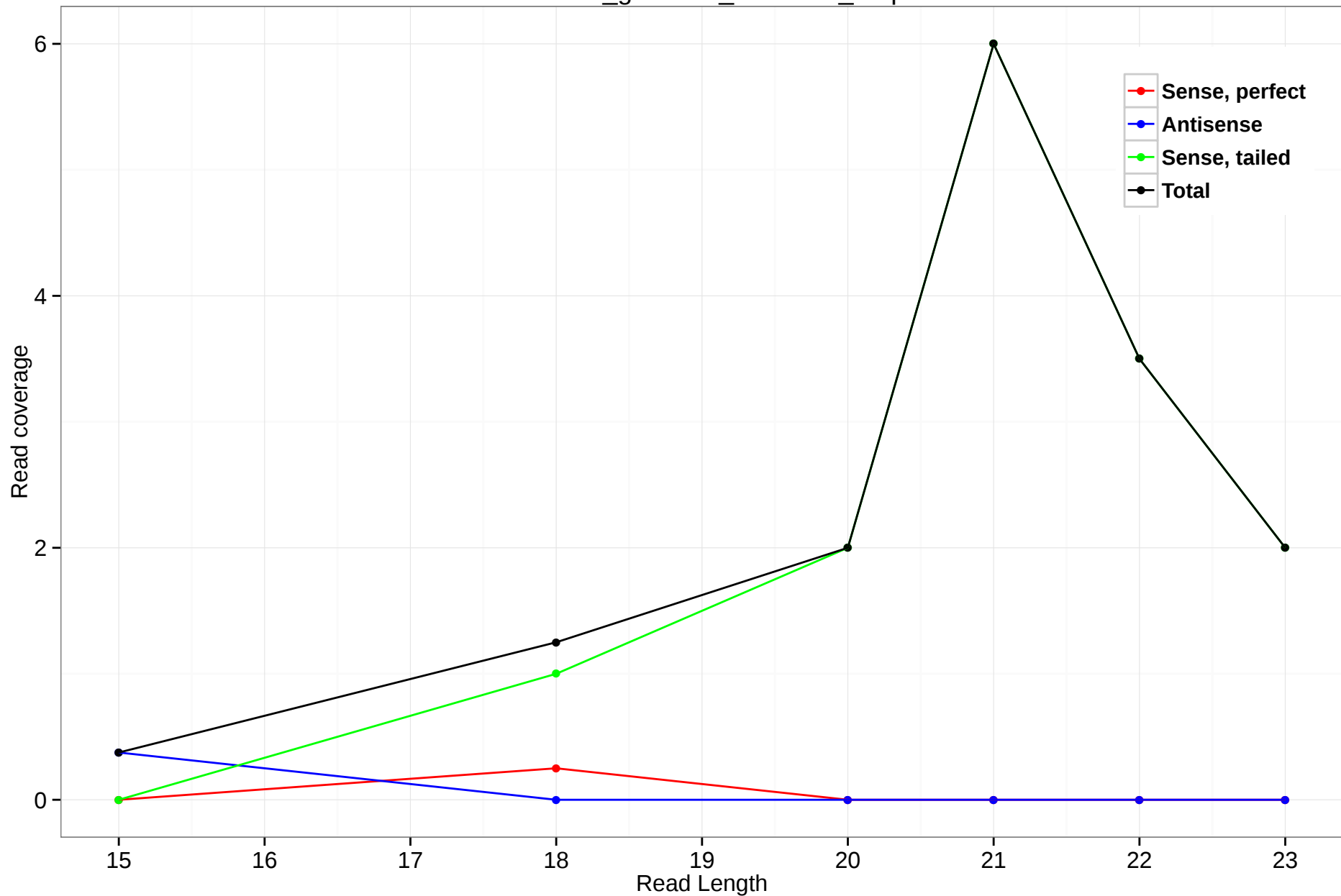
rheMac3_genscan_chr9.718_0.3p
