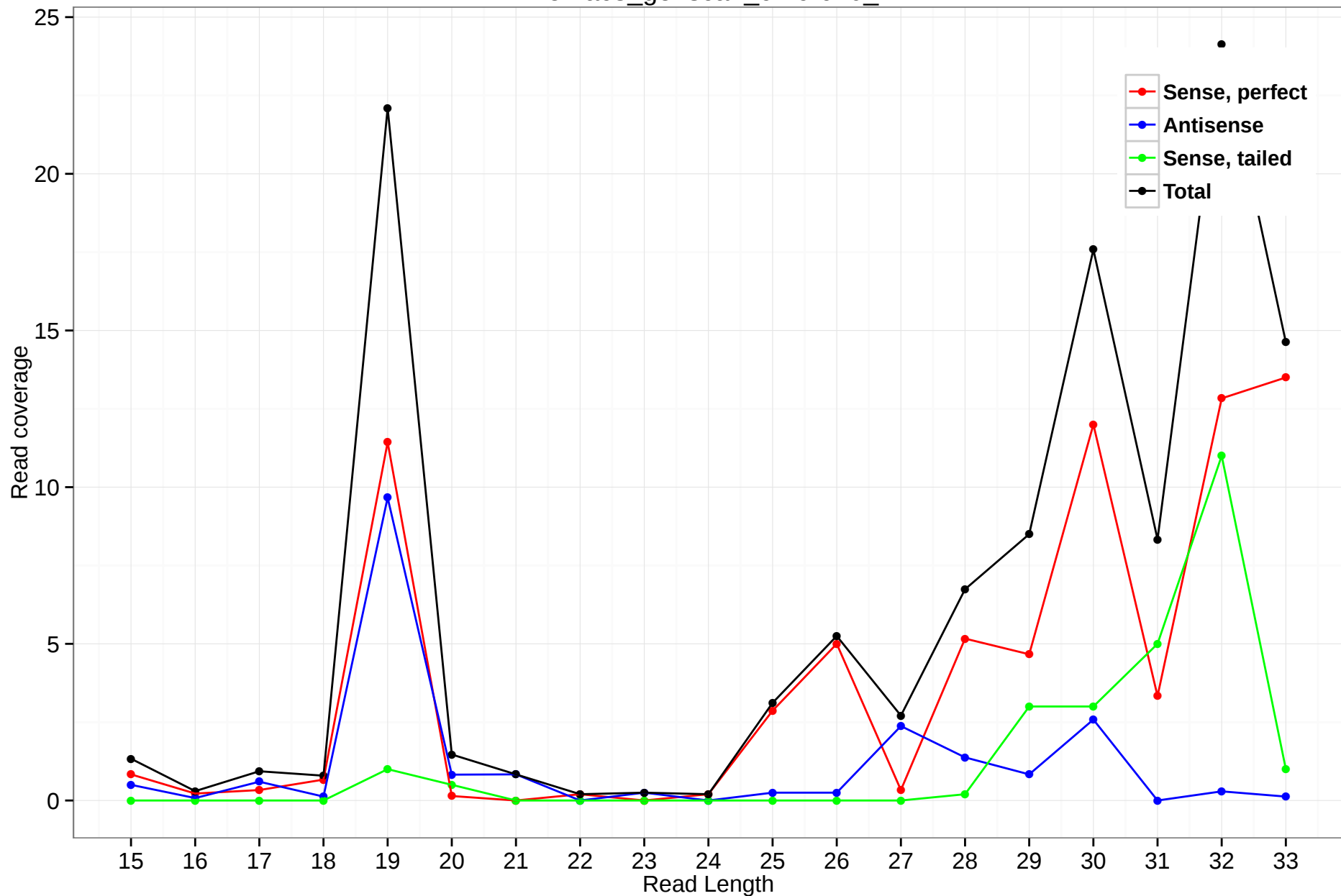
rheMac3_genscan_chr9.640_1
