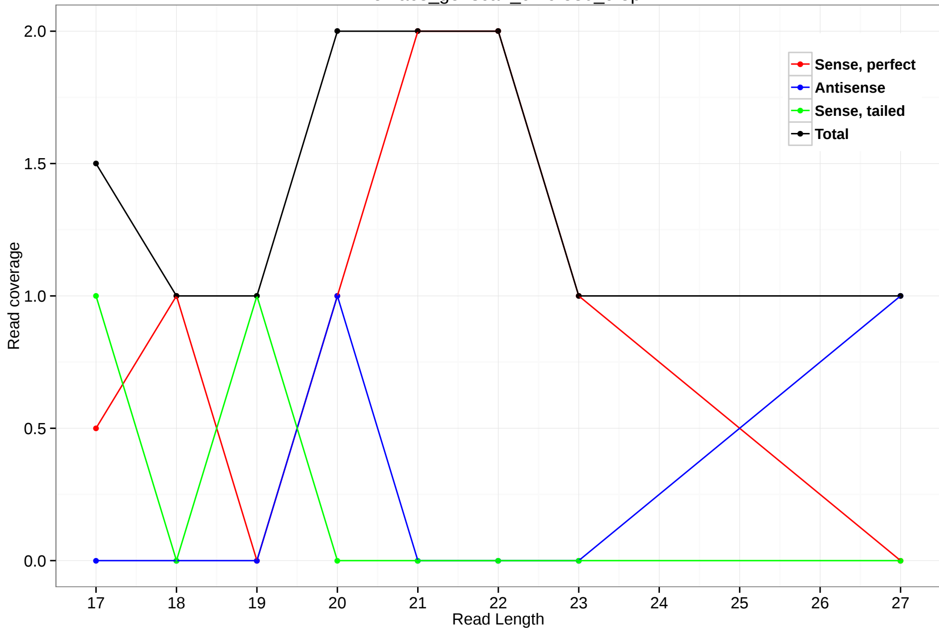
rheMac3_genscan_chr9.530_9.5p
