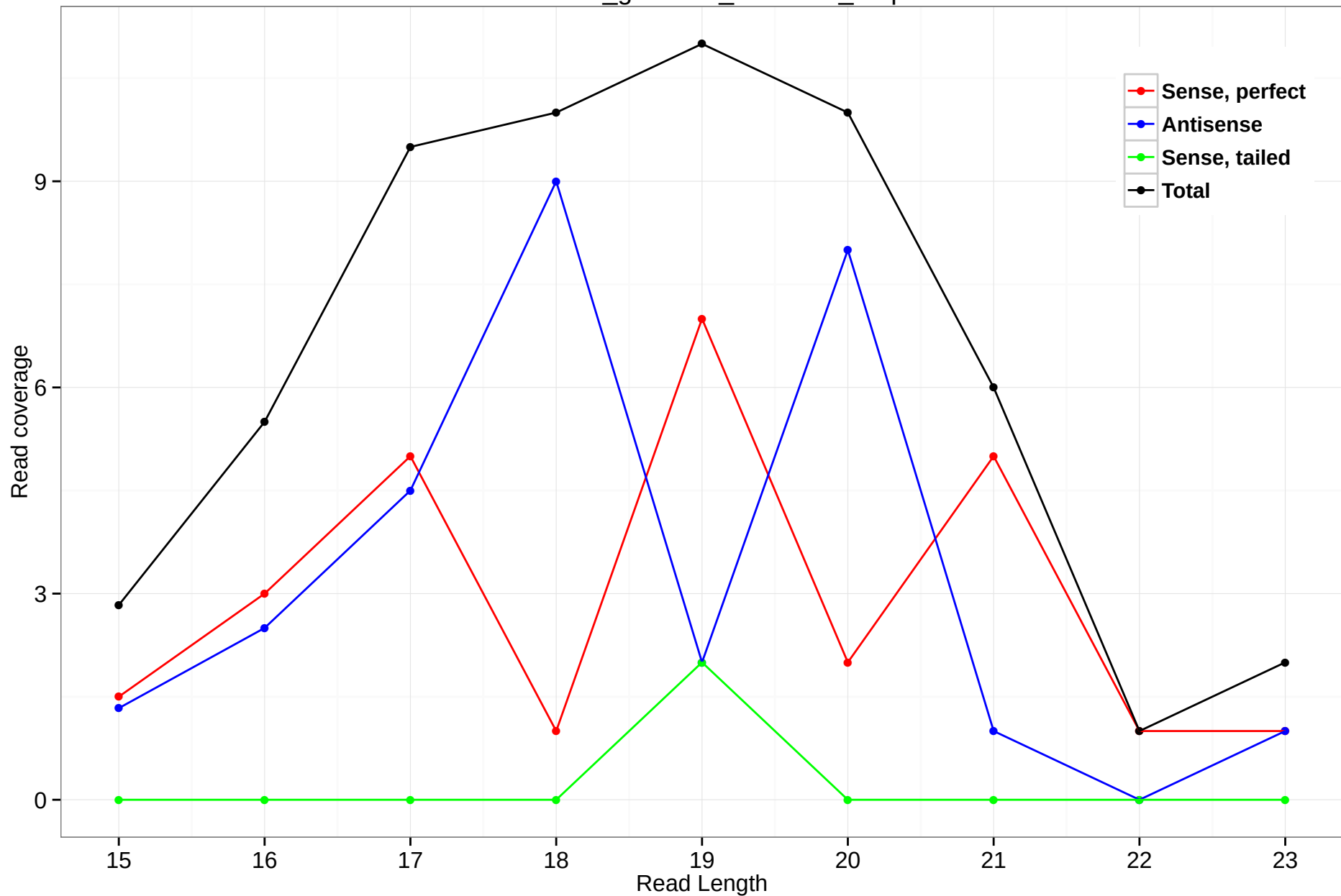
rheMac3_genscan_chr9.415_2.5p
