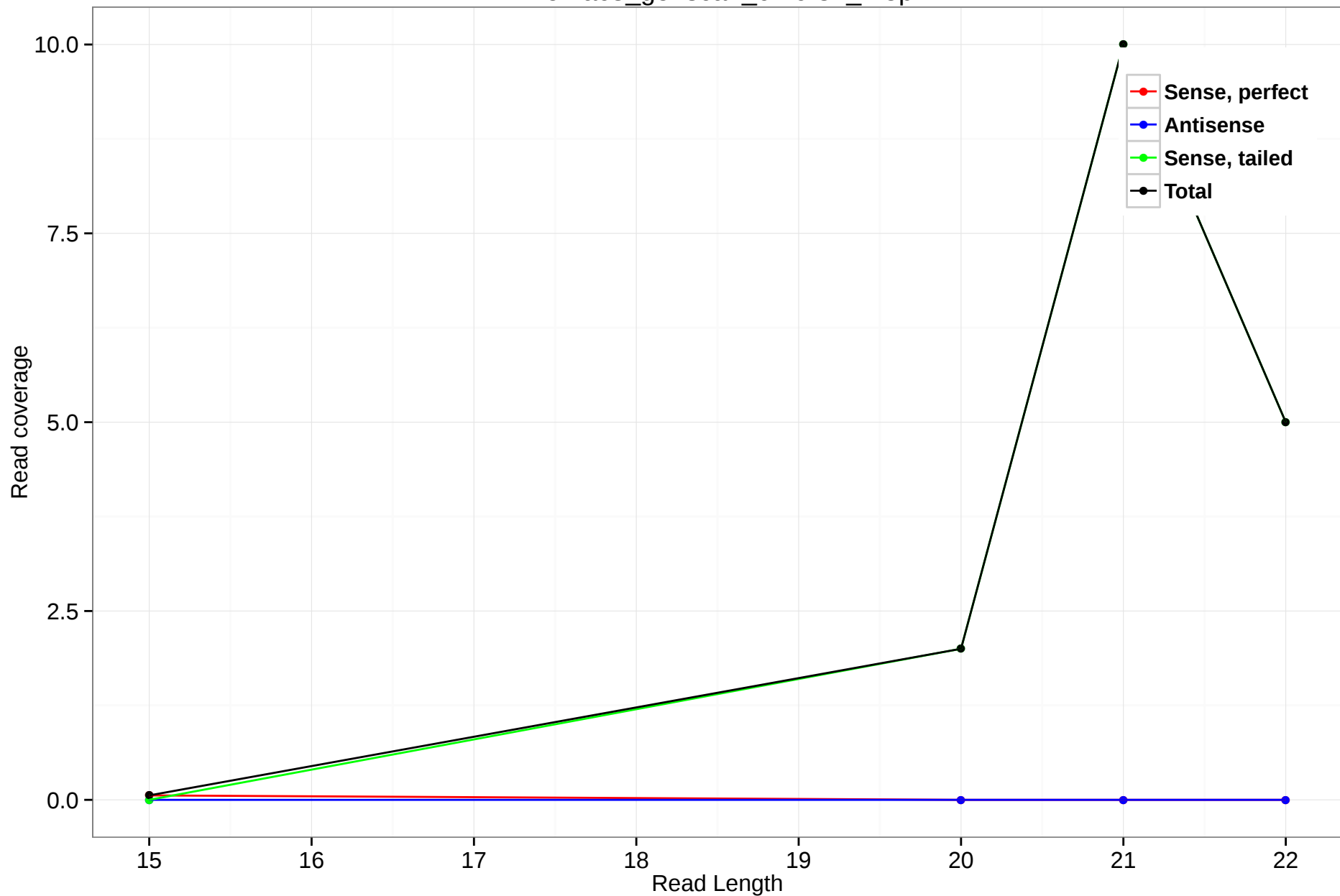
rheMac3_genscan_chr9.34_1.5p
