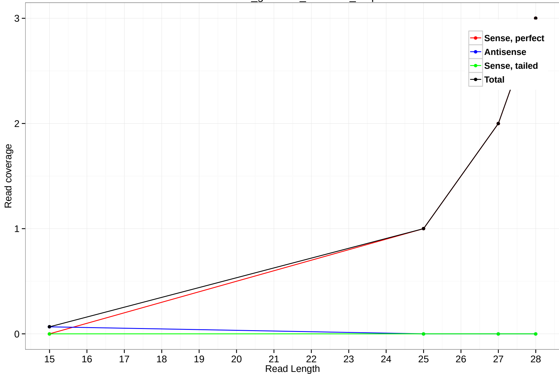
rheMac3_genscan_chr9.326_2.3p
