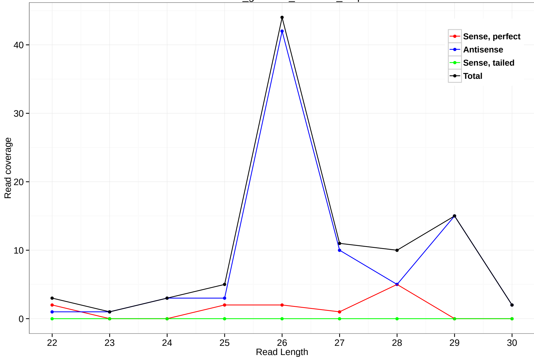
rheMac3_genscan_chr9.284_3.5p
