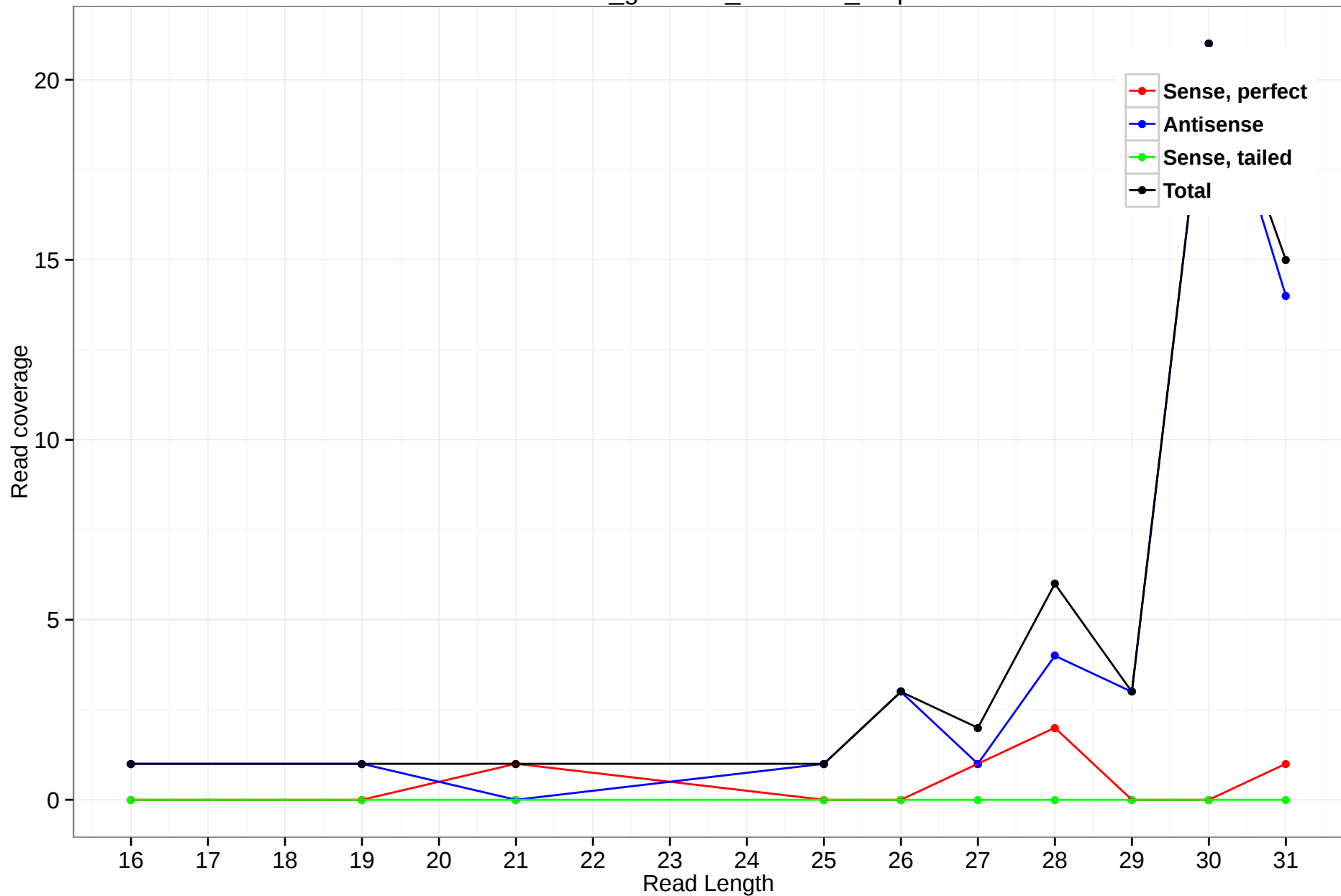
rheMac3_genscan_chr9.284_1.5p
