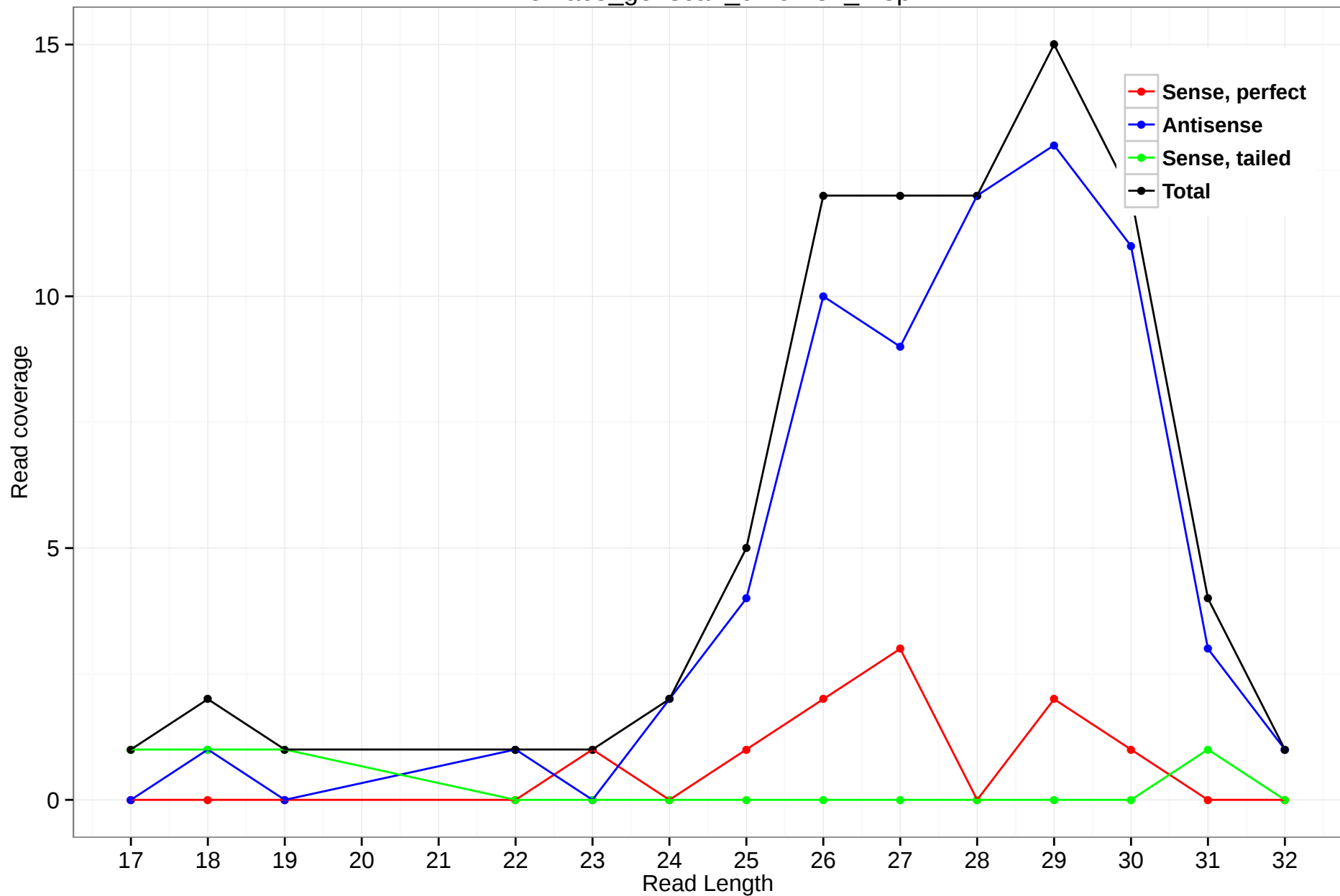
rheMac3_genscan_chr9.284_1.3p
