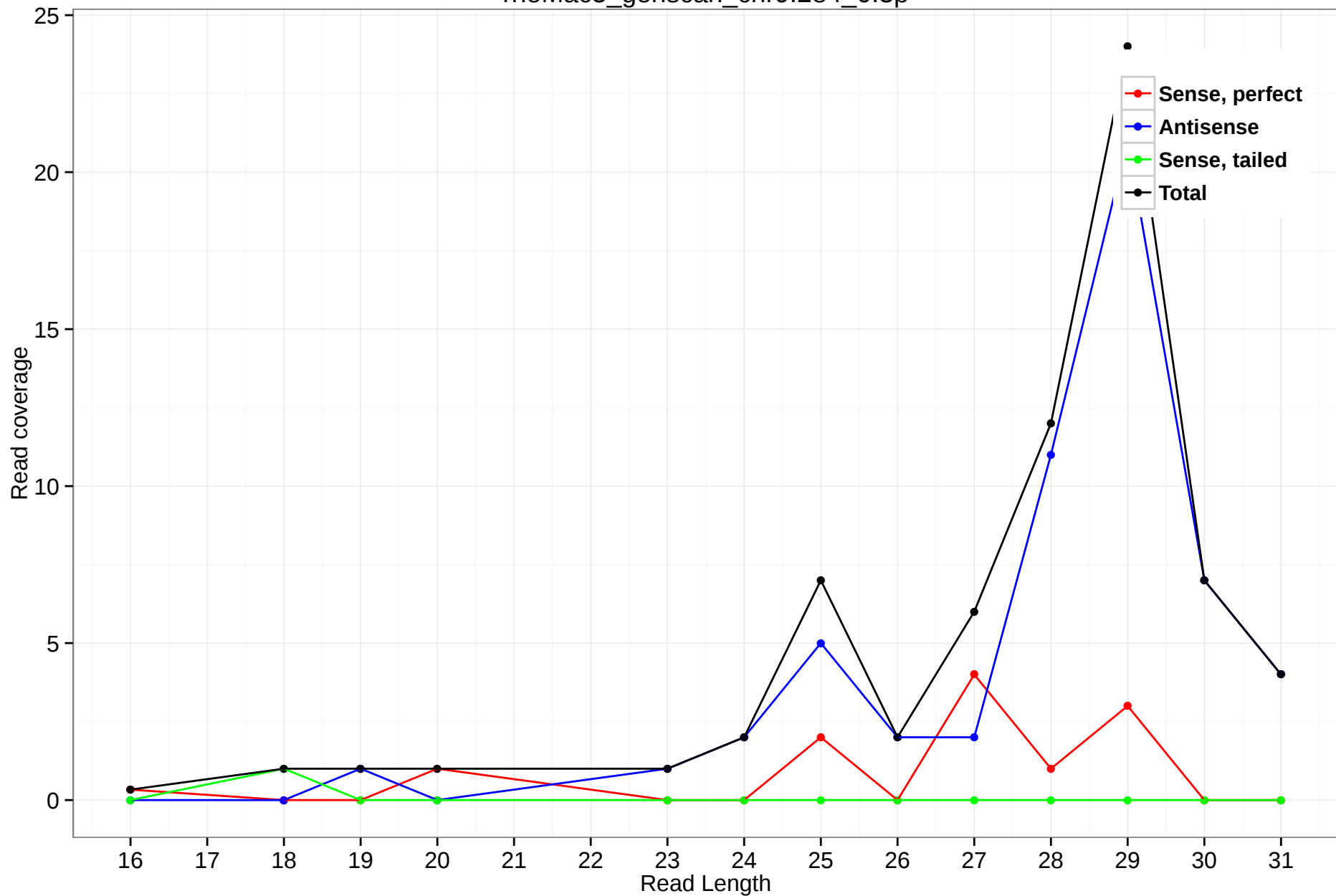
rheMac3_genscan_chr9.284_0.3p
