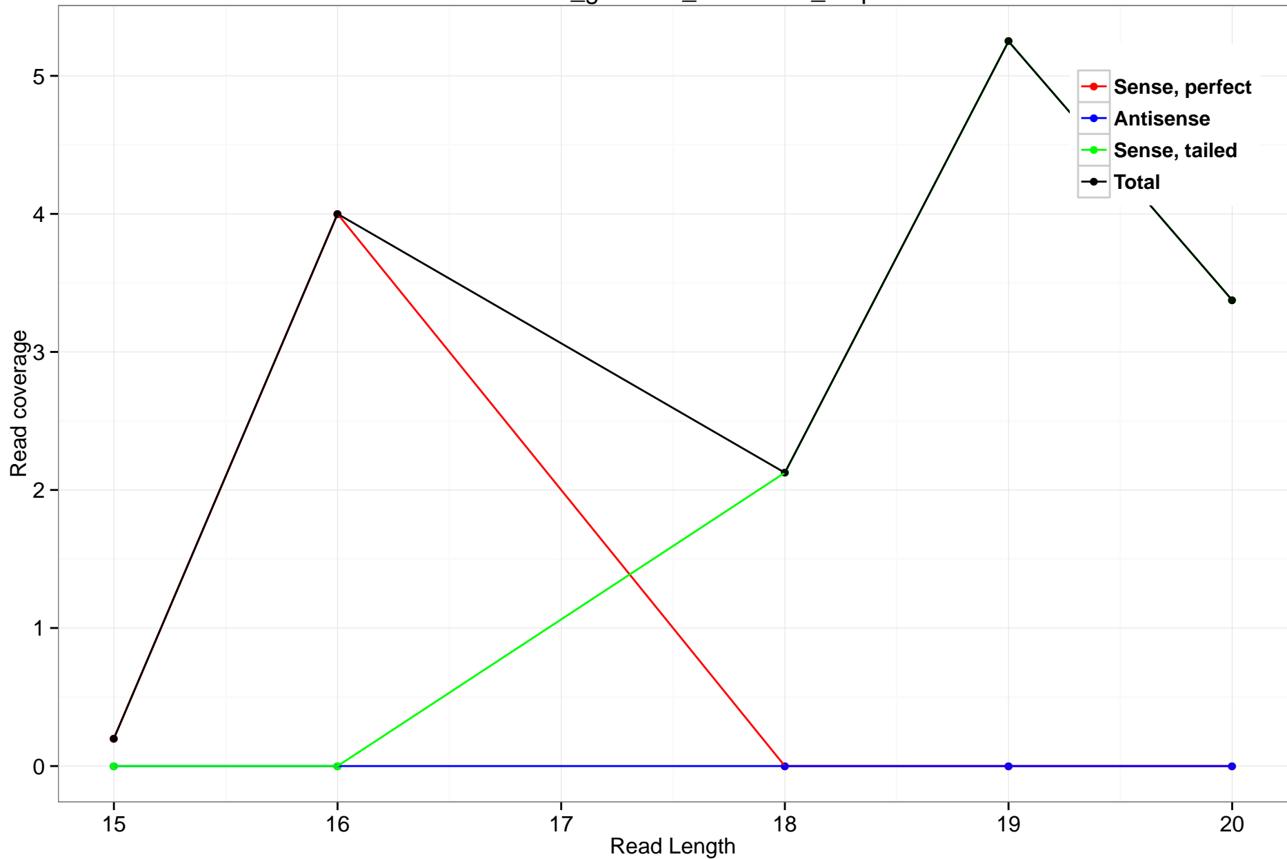
rheMac3_genscan_chr9.2696_3.5p
