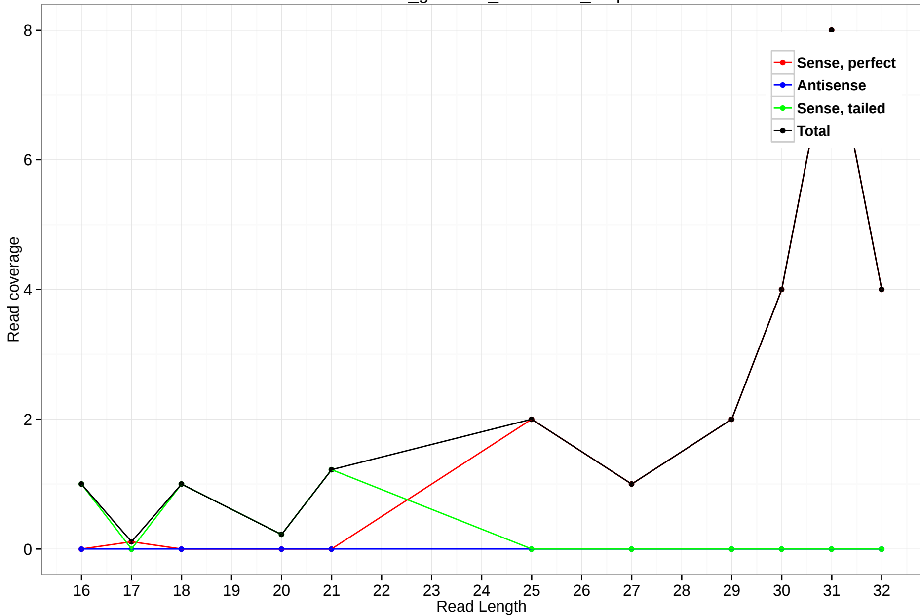
rheMac3_genscan_chr9.2690_1.5p
