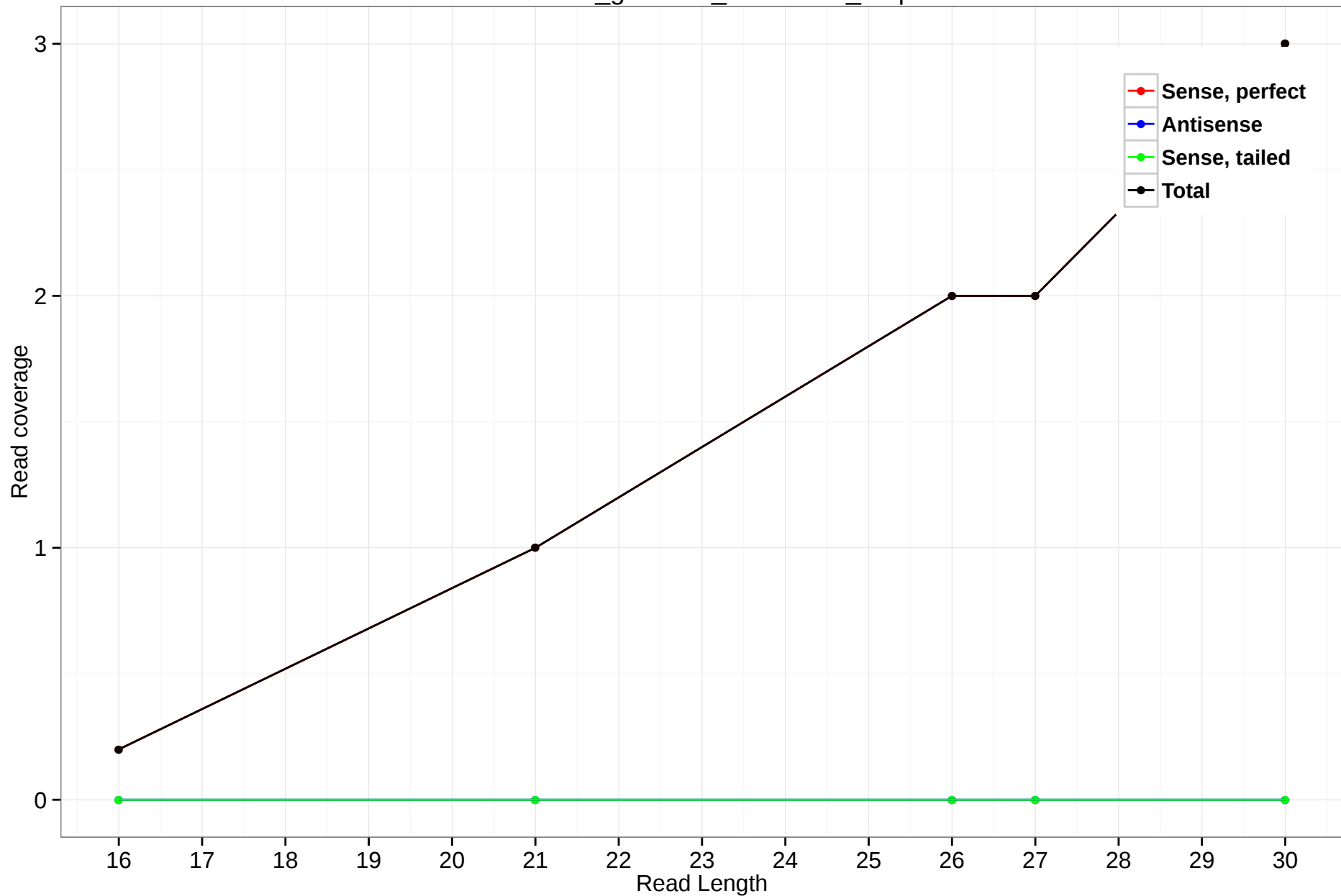
rheMac3_genscan_chr9.2566_8.3p
