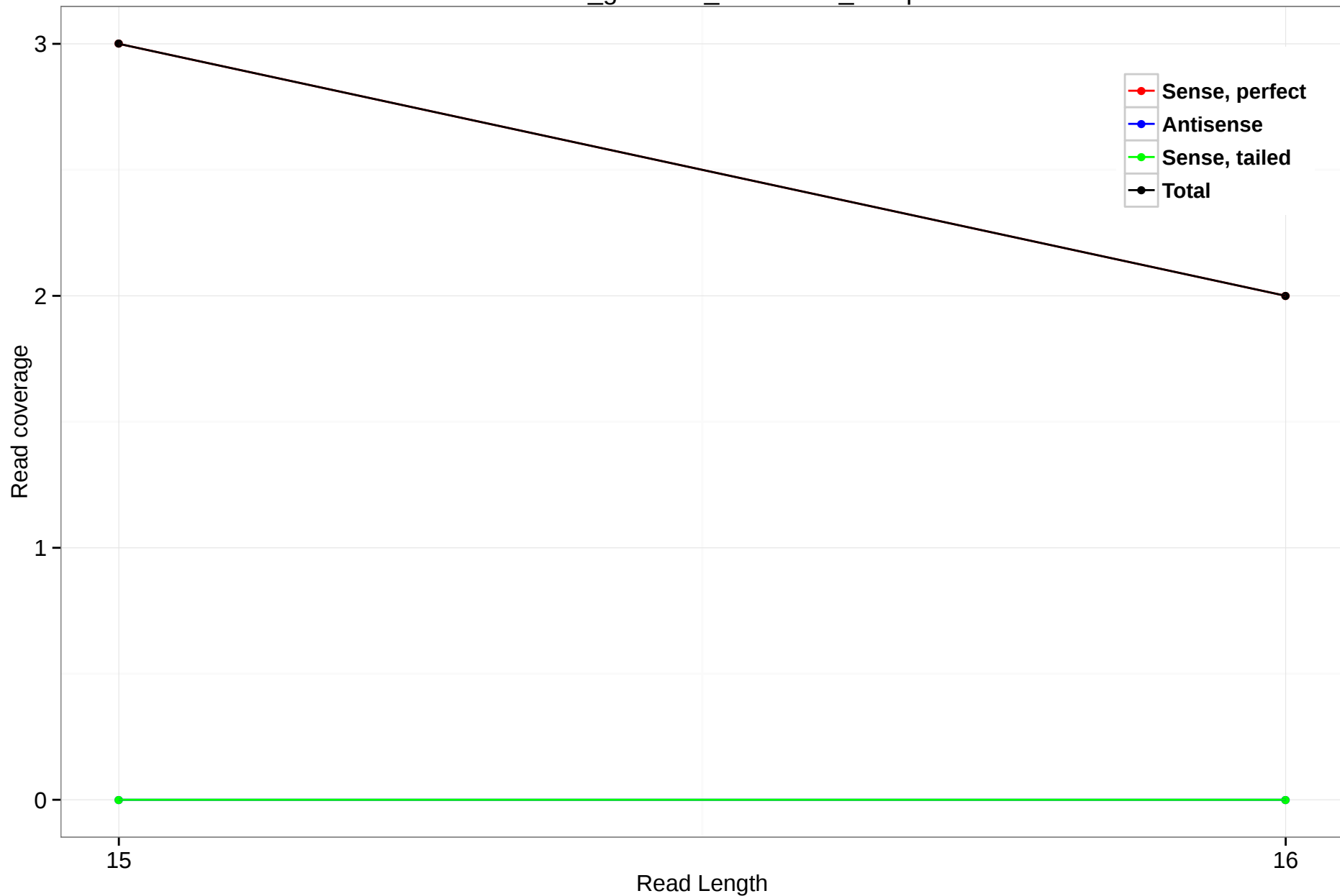
rheMac3_genscan_chr9.2548_16.3p
