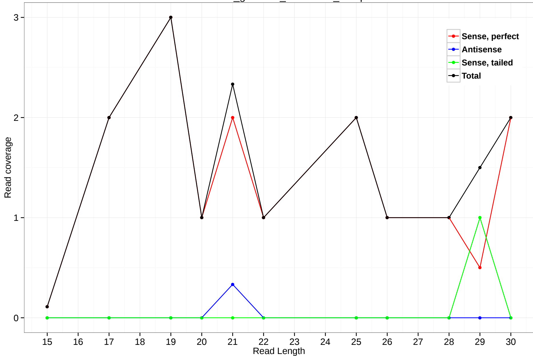
rheMac3_genscan_chr9.2408_31.5p
