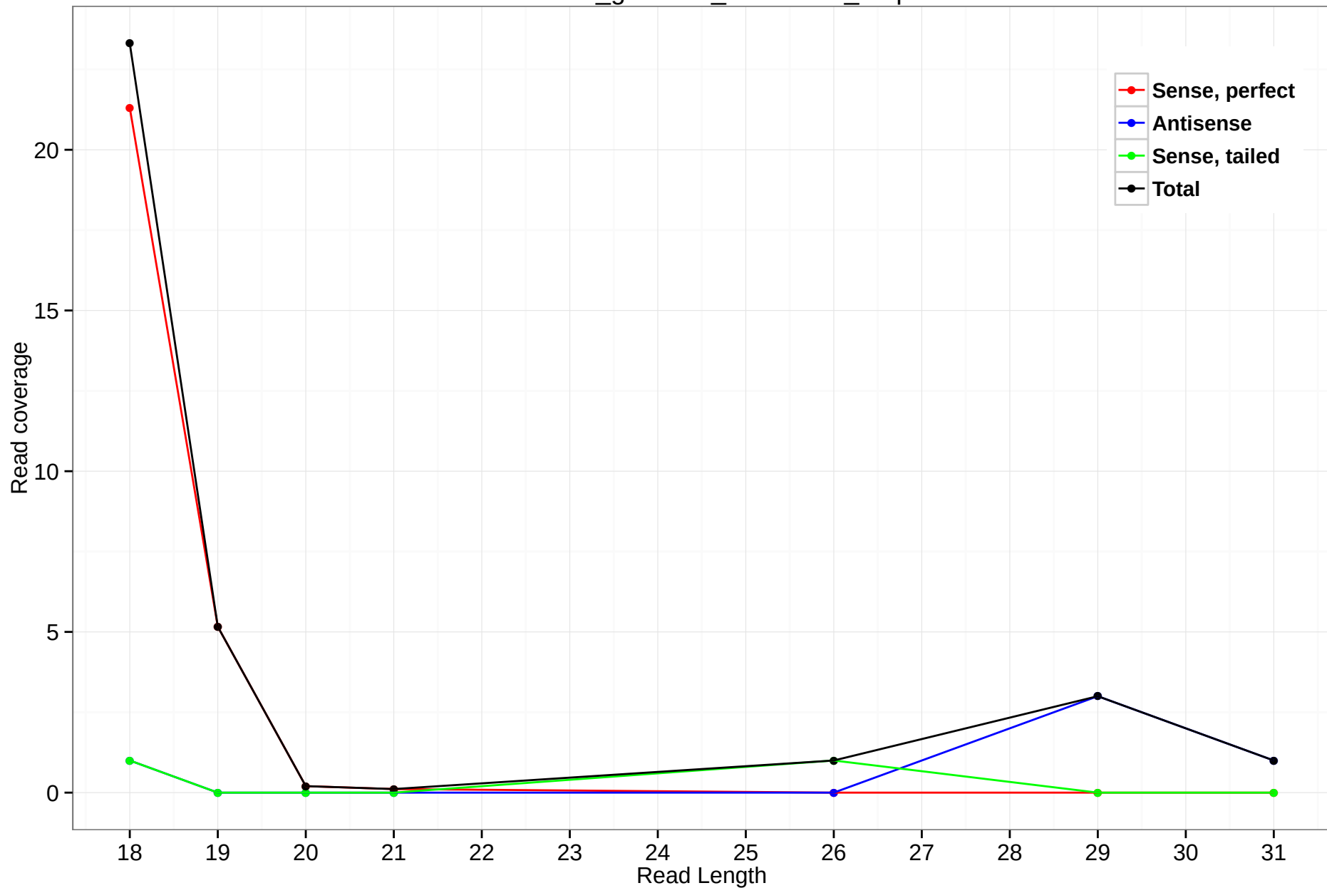
rheMac3_genscan_chr9.2376_0.3p
