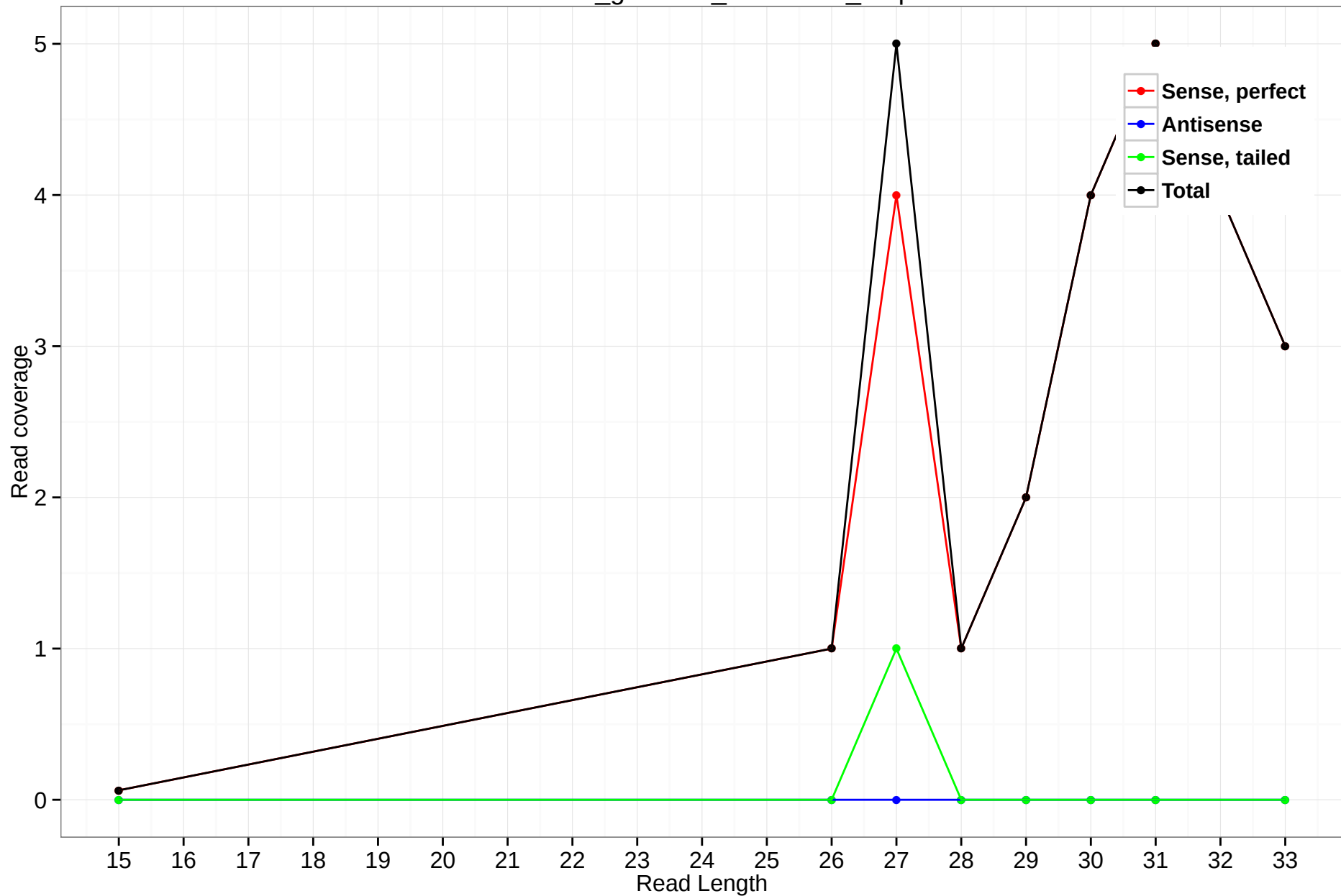
rheMac3_genscan_chr9.2276_0.5p
