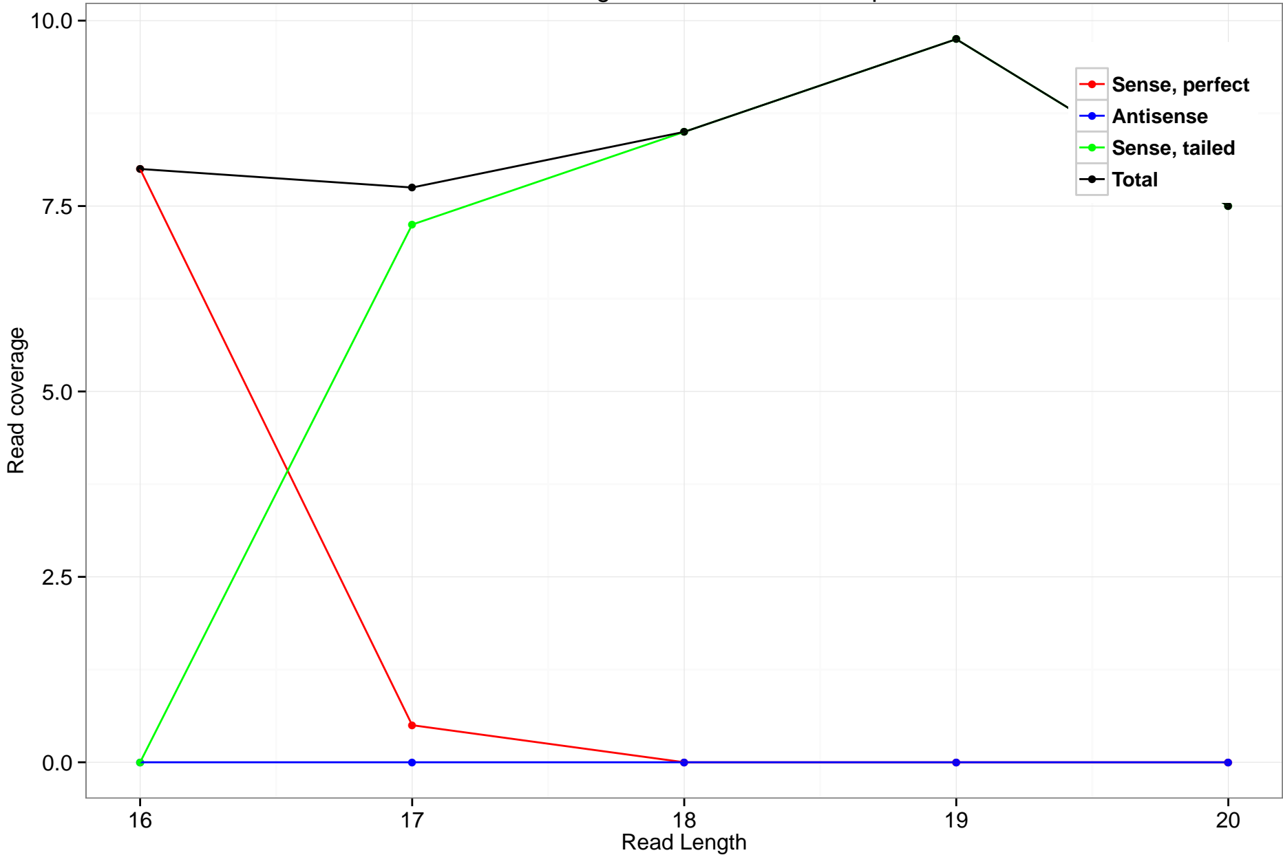
rheMac3_genscan_chr9.2270_2.5p
