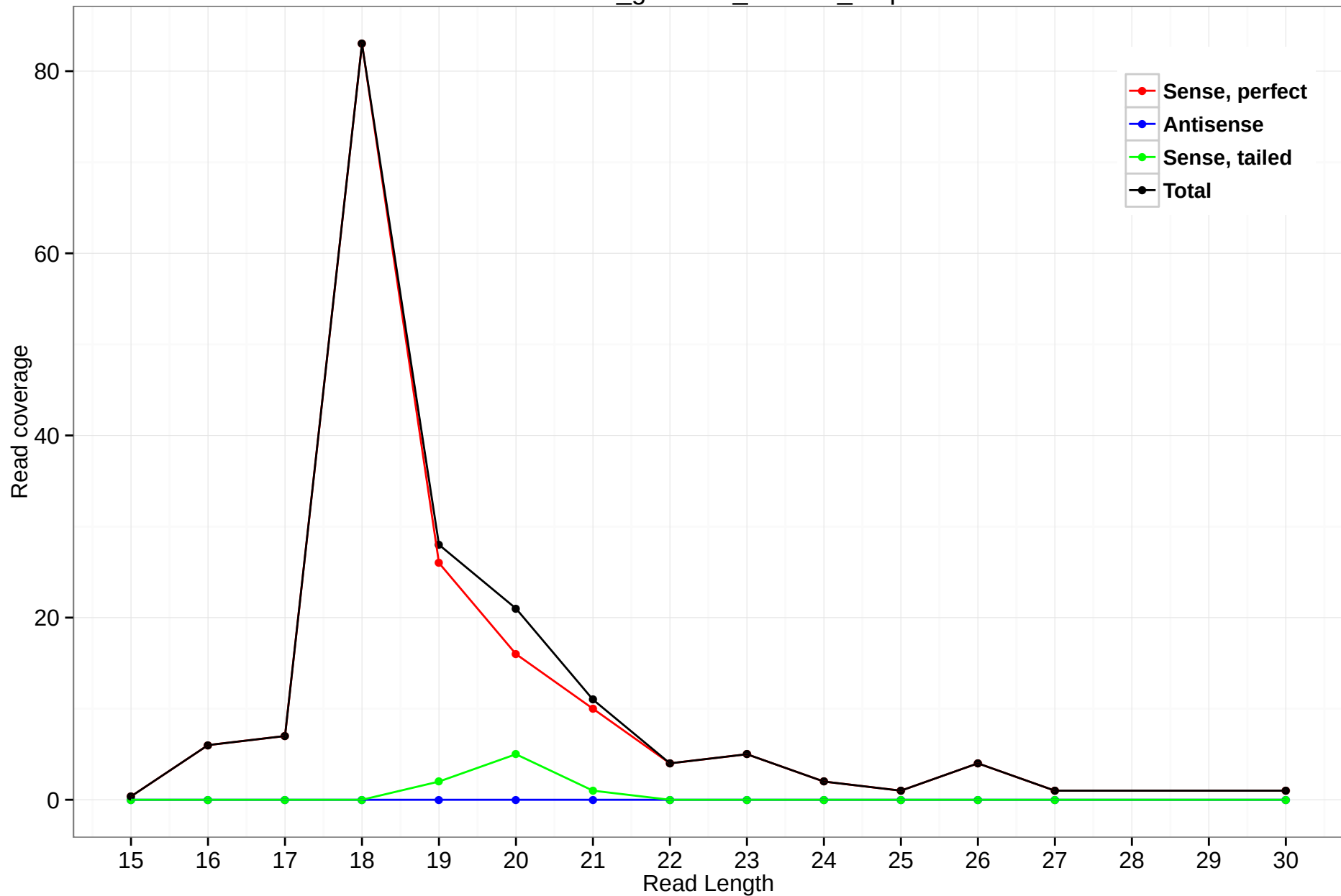
rheMac3_genscan_chr9.21_3.5p
