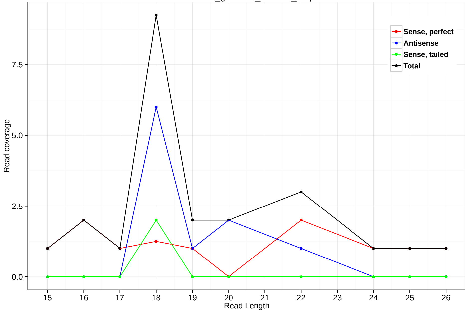
rheMac3_genscan_chr9.21_1.3p
