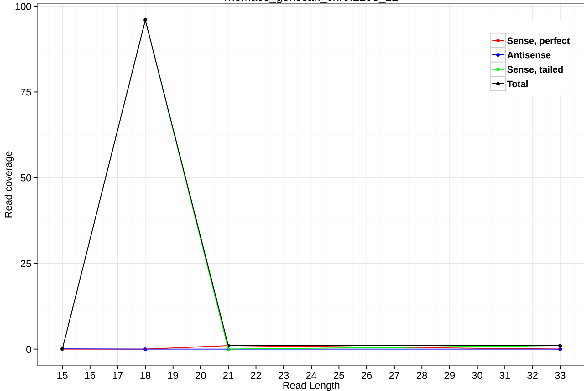
rheMac3_genscan_chr9.2193_12
