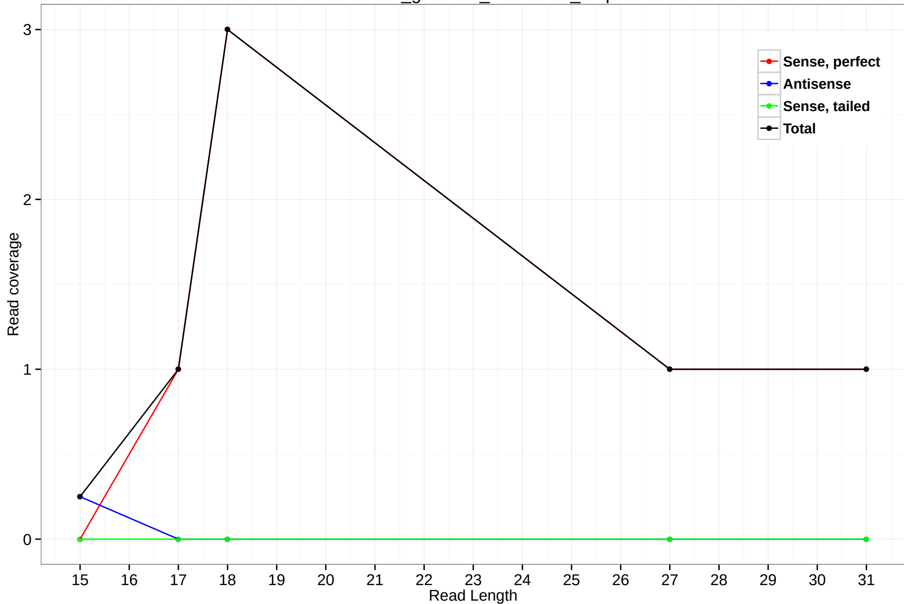
rheMac3_genscan_chr9.2158_3.3p
