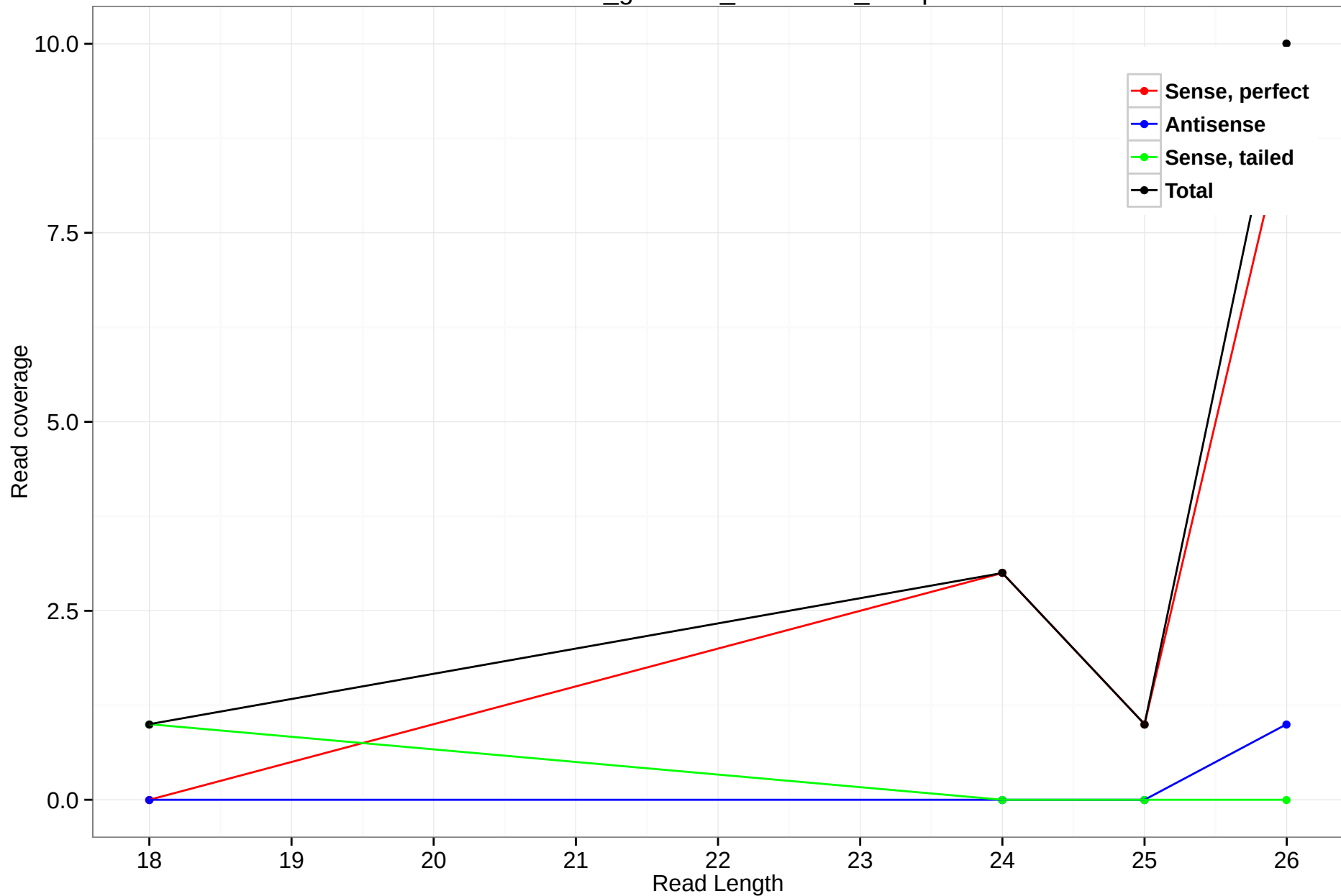
rheMac3_genscan_chr9.2051_21.5p
