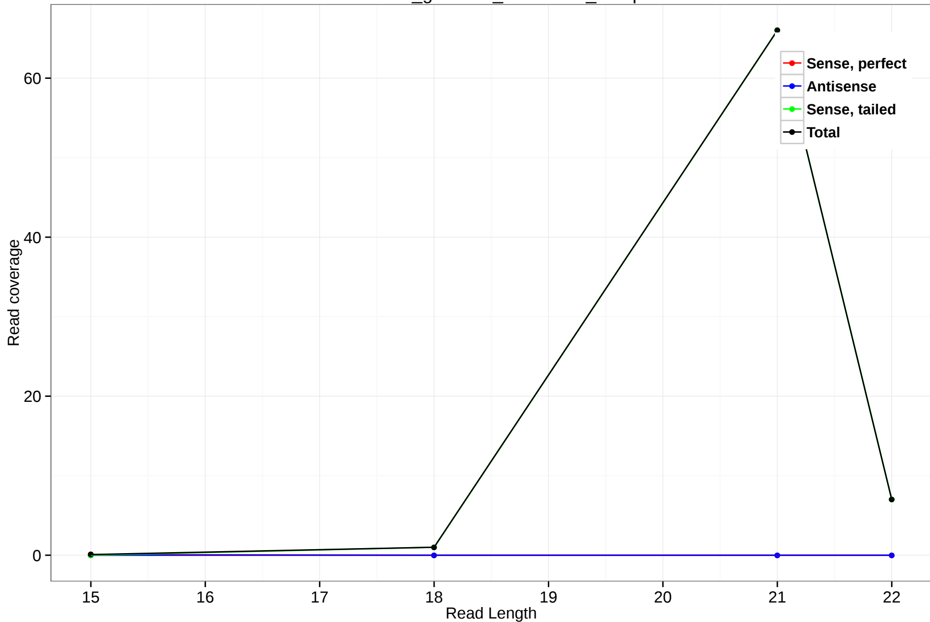
rheMac3_genscan_chr9.2046_14.5p
