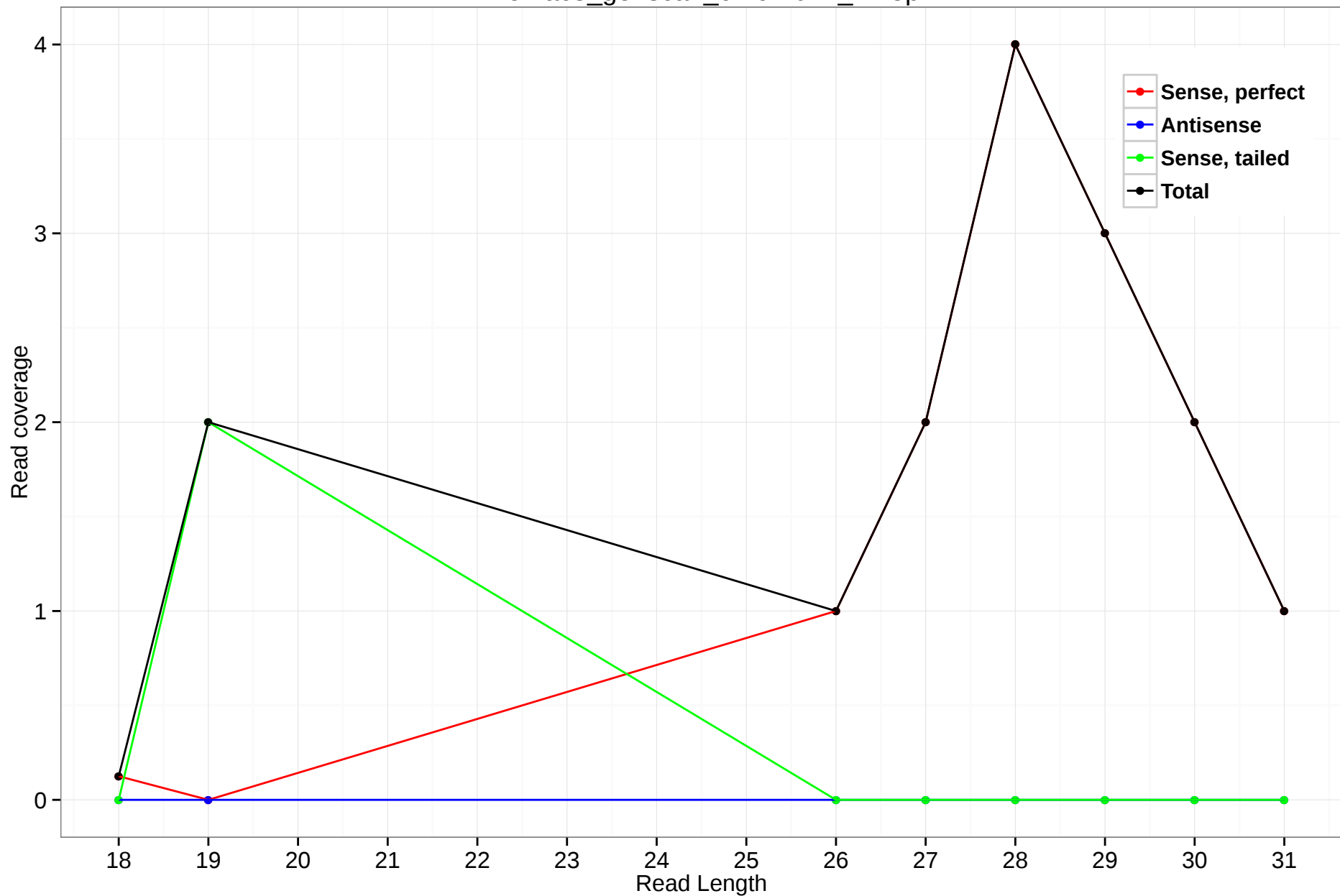
rheMac3_genscan_chr9.2042_12.5p
