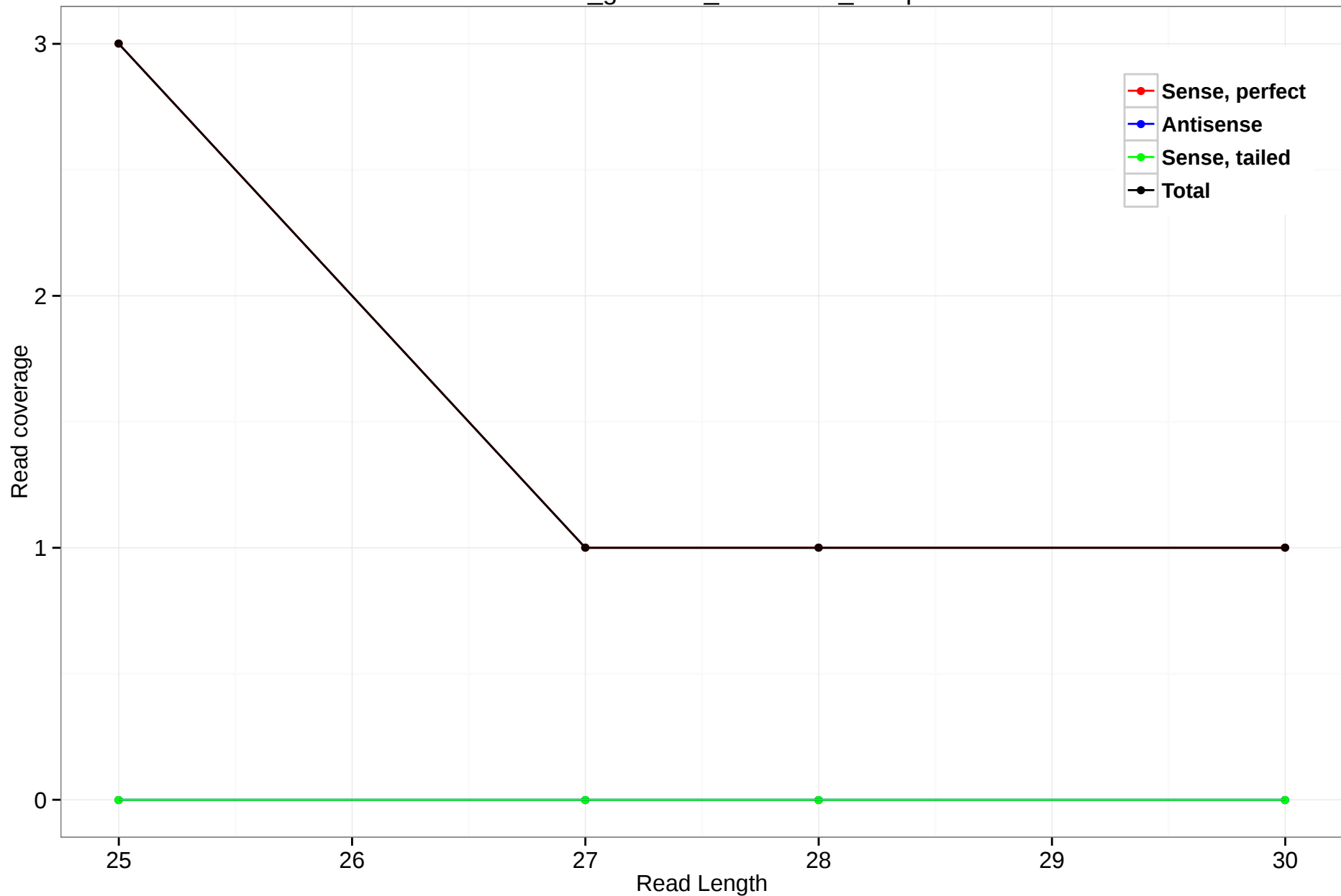
rheMac3_genscan_chr9.2041_10.5p
